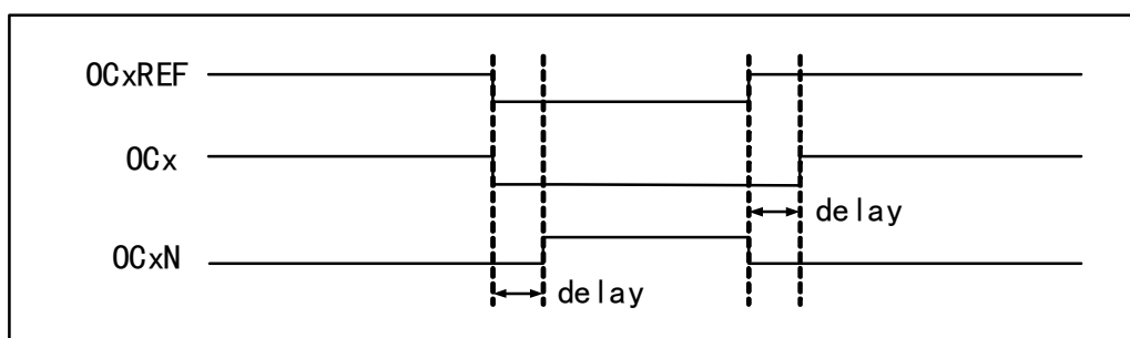
Figure 9-4 Complementary outputs and dead-time insertion
