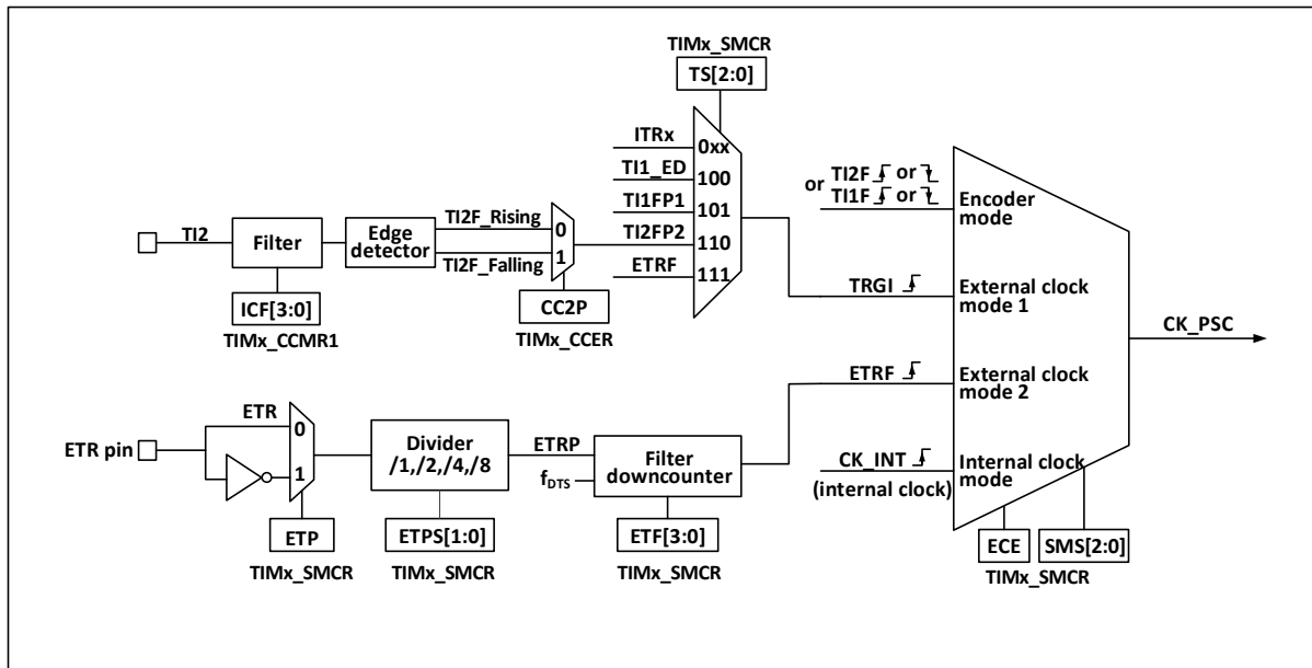
Figure 9-2 Block diagram of CK_PSC source for advanced-control timer
