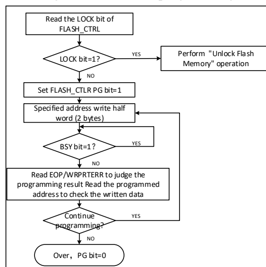
Figure 14-1 FLASH programming
