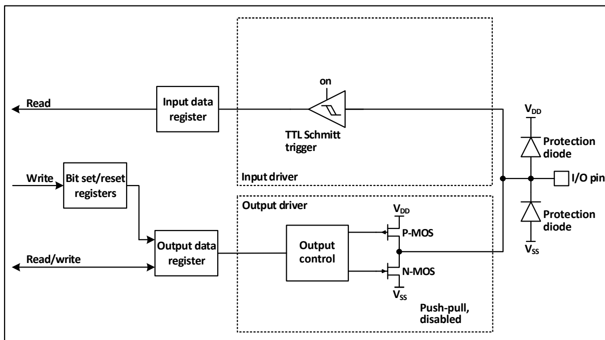
Figure 6-3 GPIO module output configuration structure block diagram
