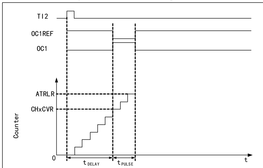
Figure 9-5 Generation of one pulse mode
