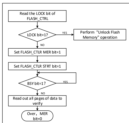
Figure 14-3 FLASH whole chip erase
