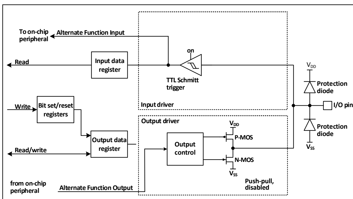
Figure 6-4 The structure of GPIO module when it is alternate by other peripherals
