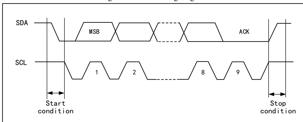
Figure 12-1 I2C timing diagram
