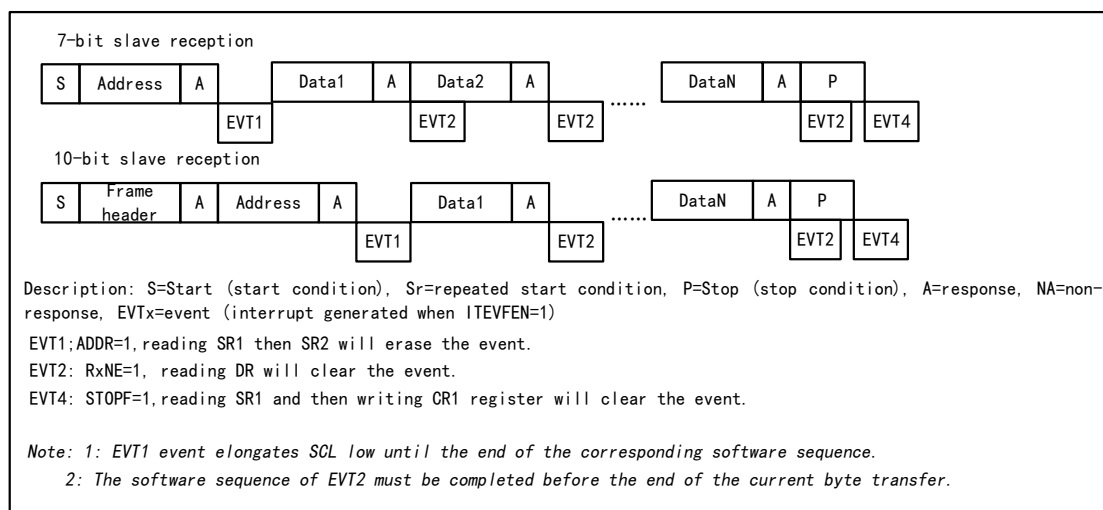
Figure 12-4 Receiver transmission sequence diagram
