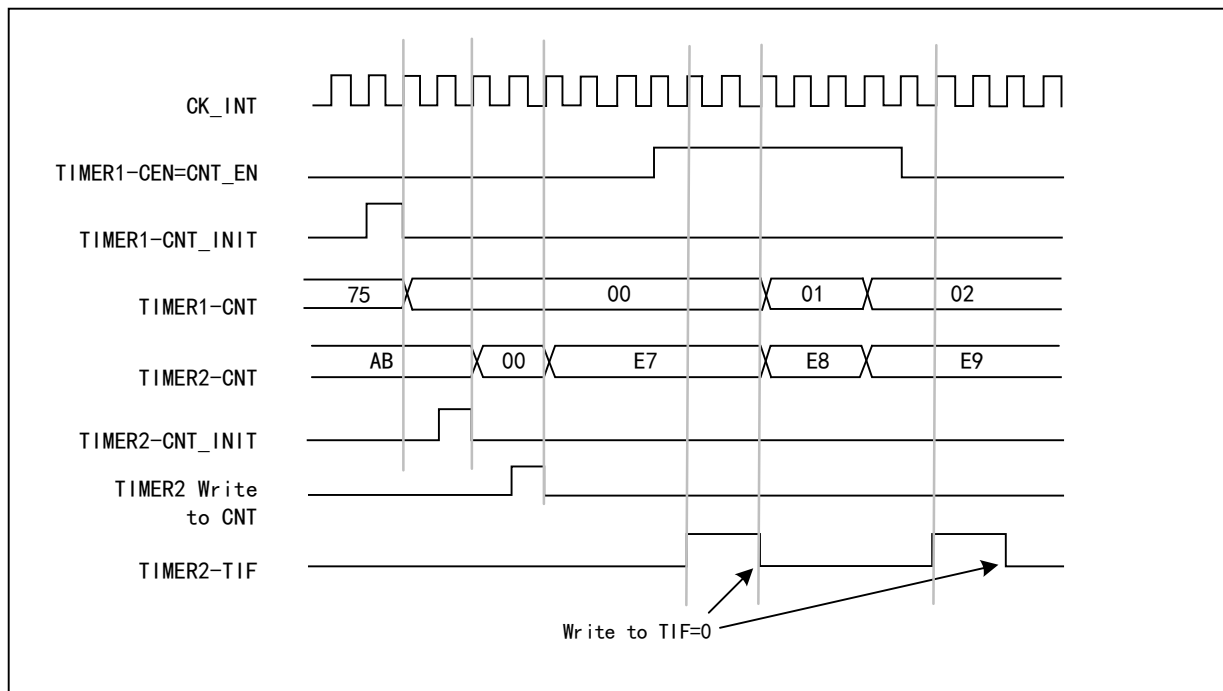
Figure 12-12 Gating Timer 2 using Timer 1's enable signal
