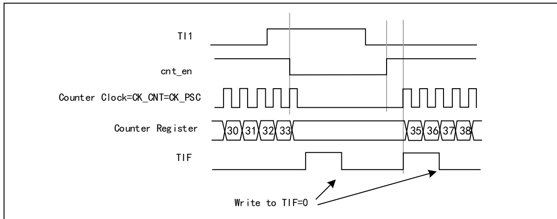
Figure 13-6 Control circuit in gated mode
