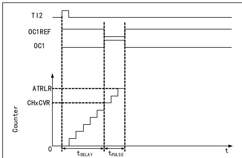
Figure 13-4 Event generation and impulse response
