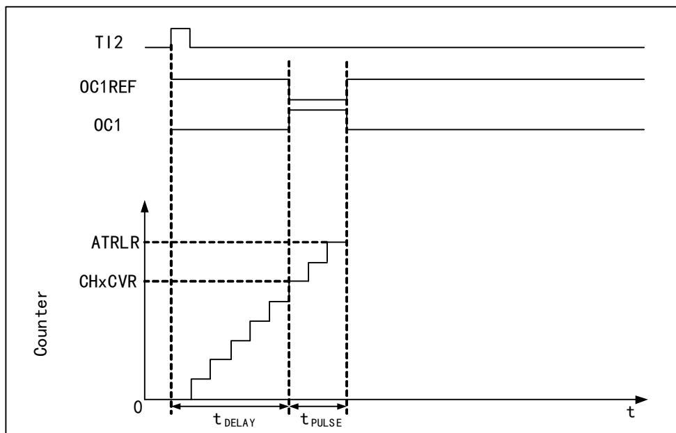
Figure 12-5 Generation of one pulse mode
