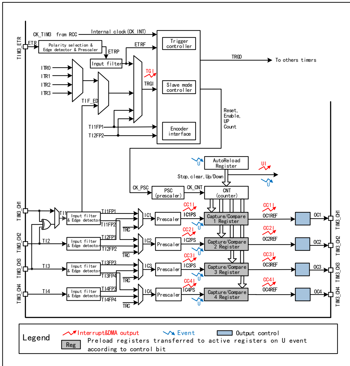
Figure 13-1 Block diagram of the structure of the general-purpose timer
