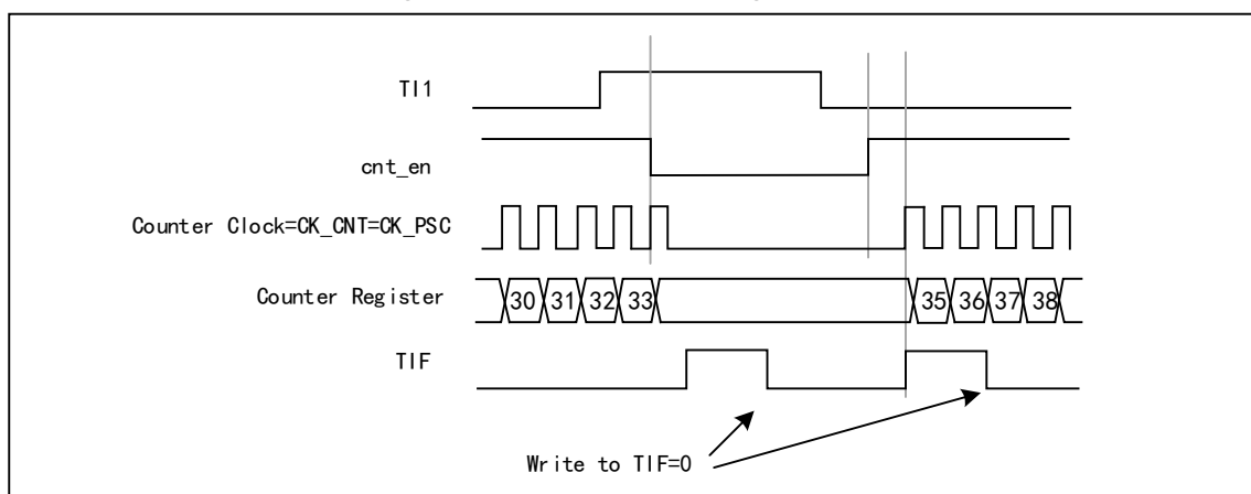
Figure 12-7 Control circuit in gated mode
