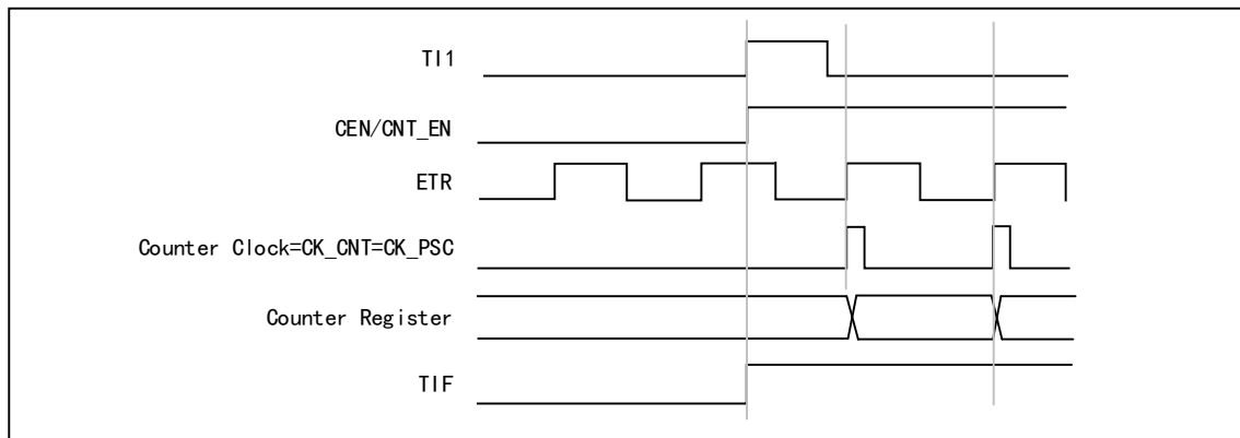
Figure 12-9 Control circuit in external clock mode 2 + trigger mode
