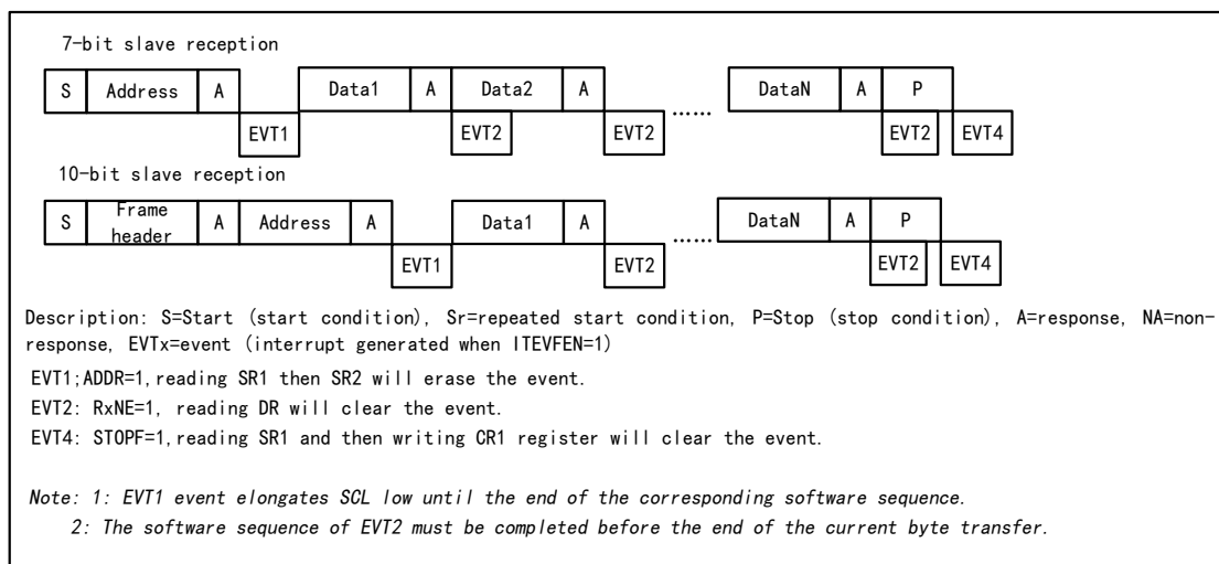
Figure 15-6 Receiver transmission sequence diagram
