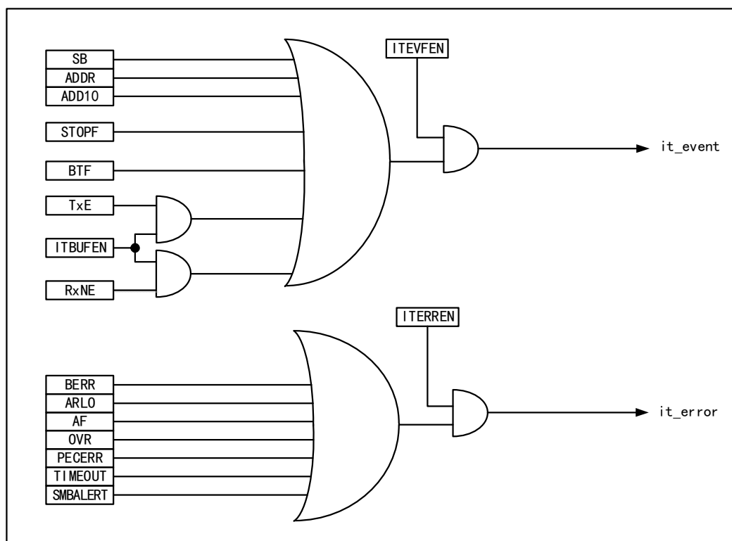
Figure 15-7 I2C Interrupt Request
