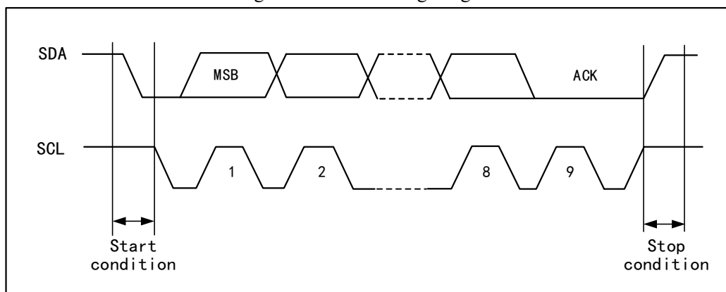
Figure 15-1 I2C Timing Diagram
