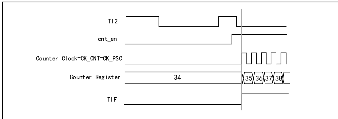
Figure 12-8 Control circuit in trigger mode
