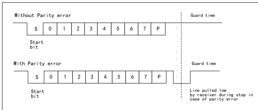
Figure 14-4 (Un)Occurrence of parity error diagram
