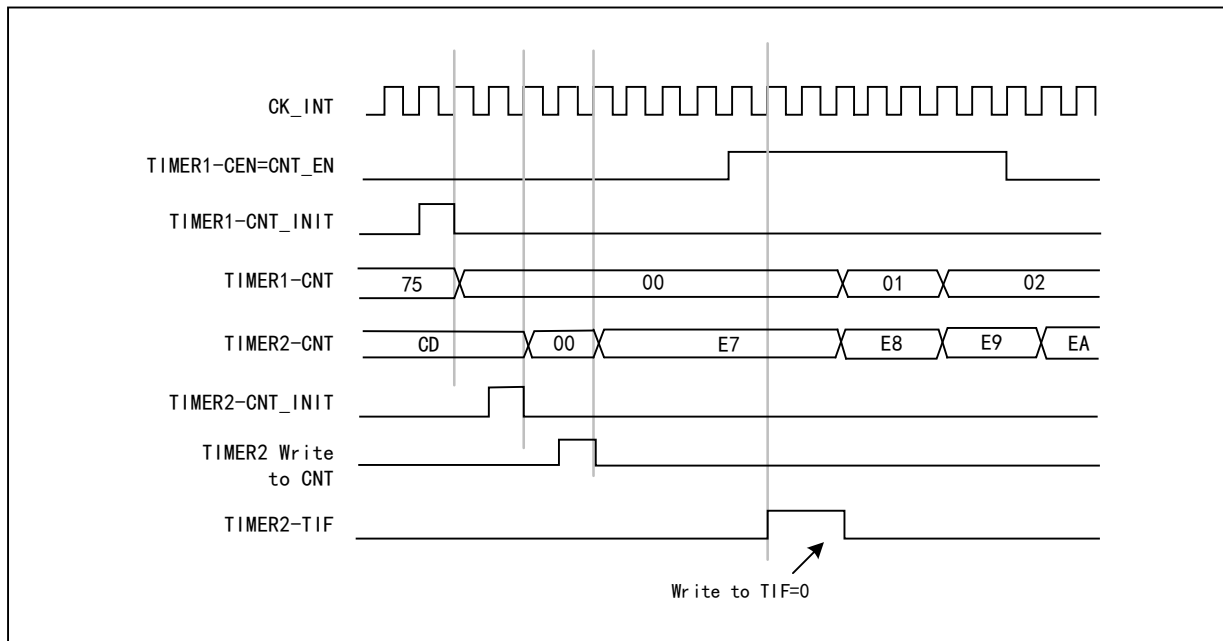
Figure 12-14 Triggering Timer 2 using Timer 1's enable signal
