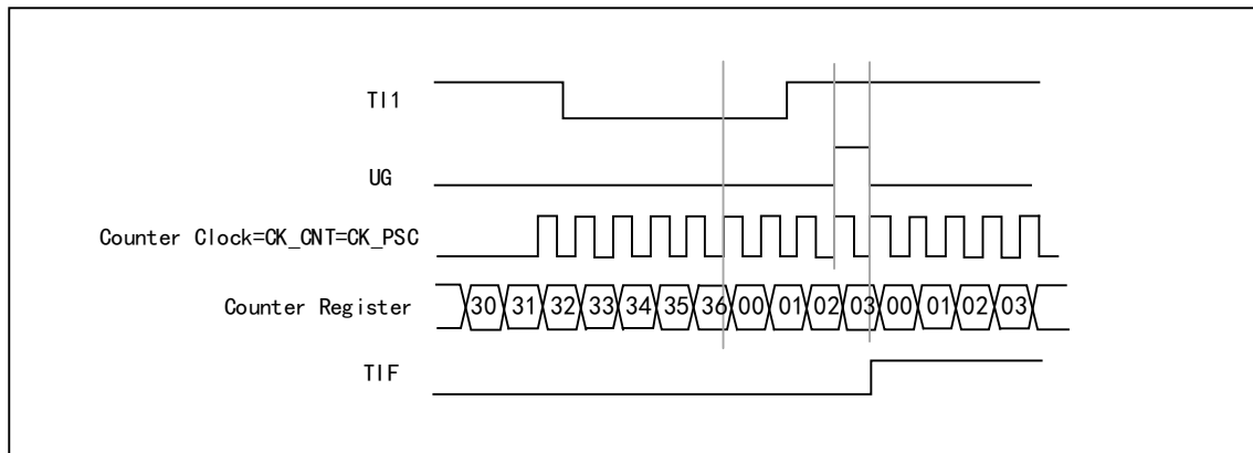
Figure 12-6 Control circuit in reset mode
