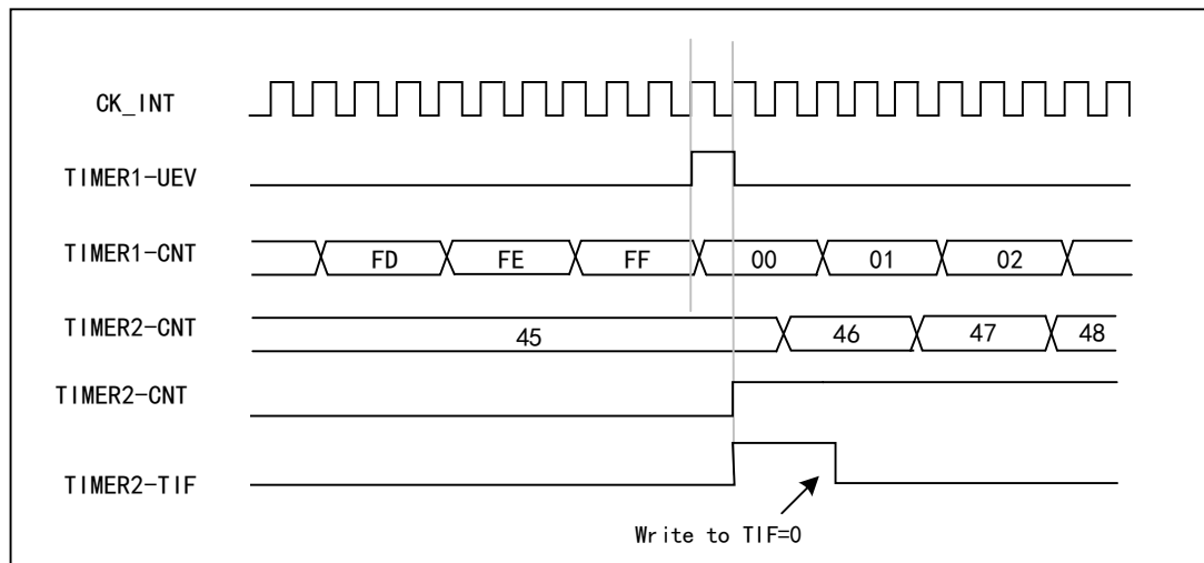
Figure 12-13 Triggering Timer 2 using Timer 1 update event
