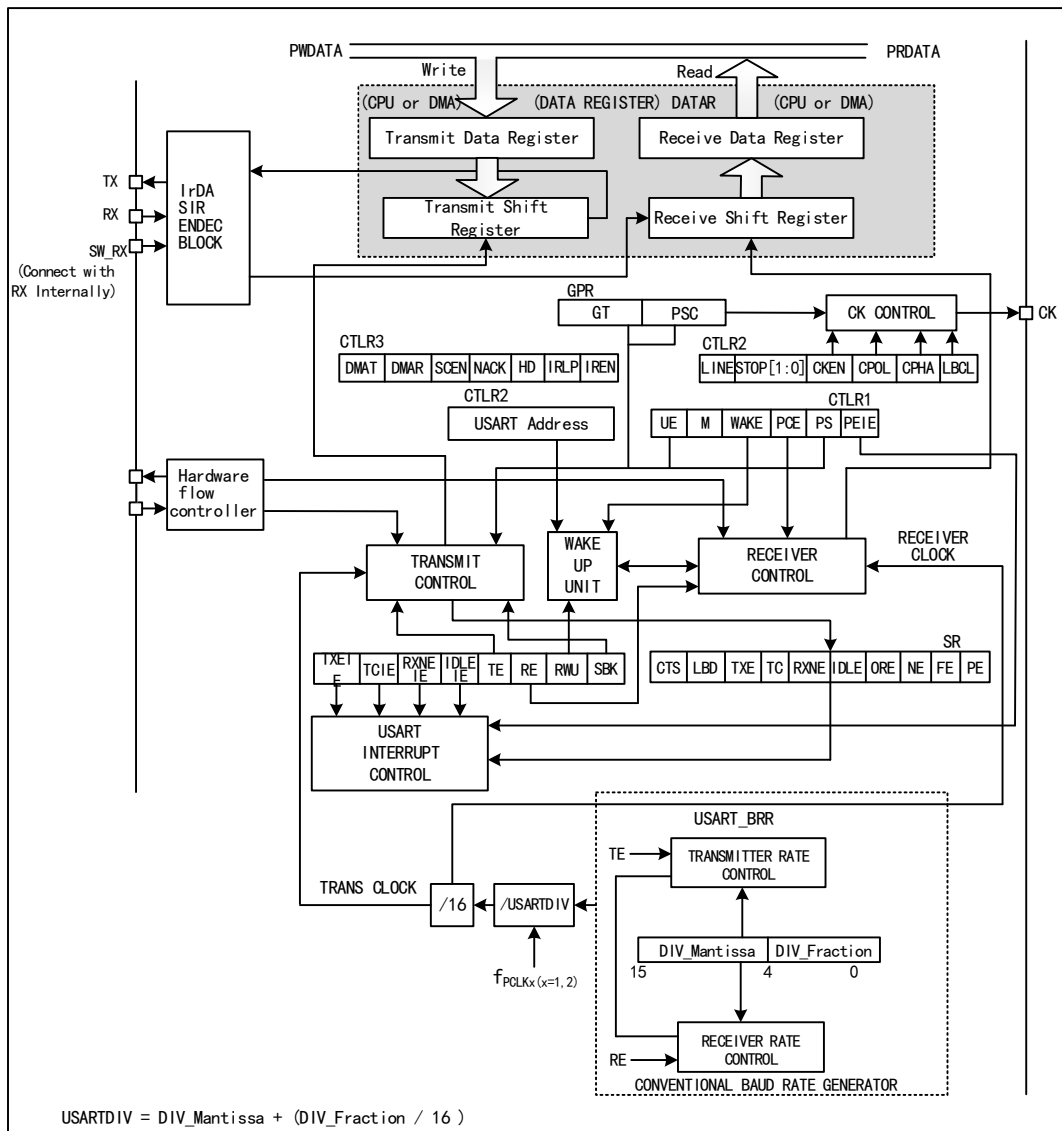
Figure 14-1 Block diagram of a general-purpose synchronous/asynchronous transceiver
