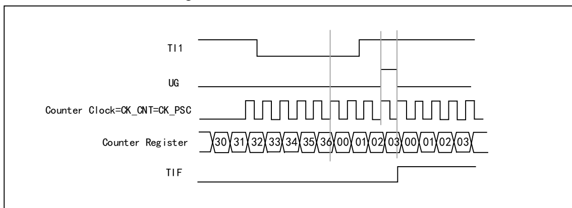
Figure 13-5 Control circuit in reset mode
