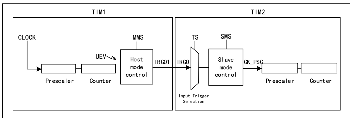
Figure 12-10 Master/slave timer example
