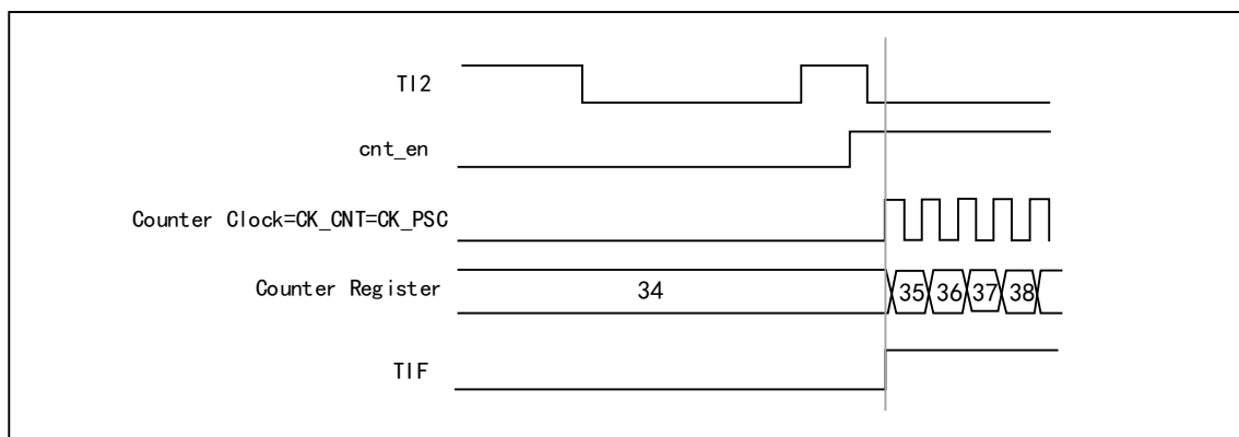
Figure 13-7 Control circuit in trigger mode
