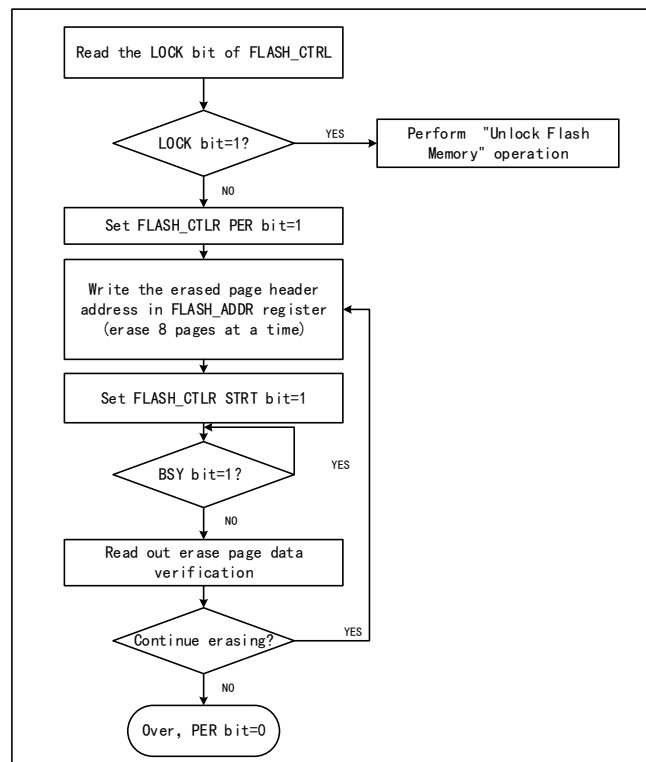
Figure 20-1 FLASH page erase
