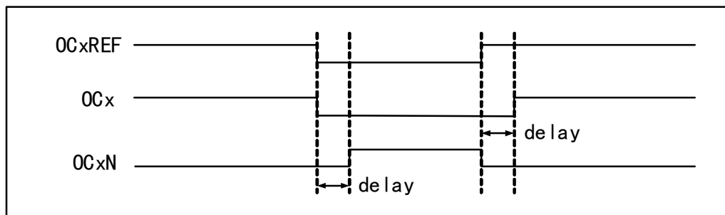
Figure 12-4 Complementary outputs and dead-time insertion
