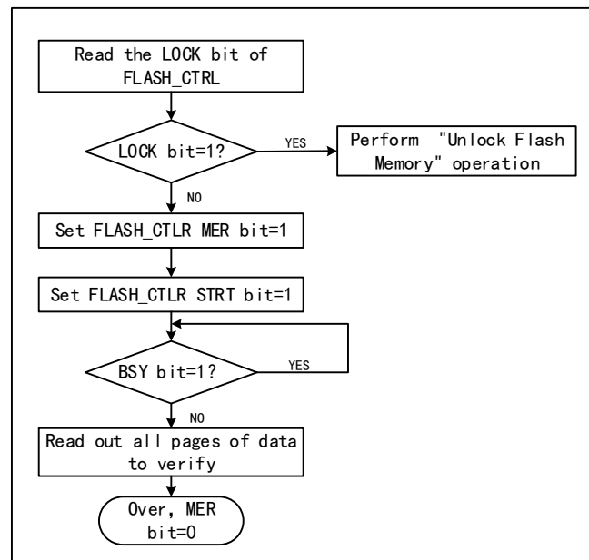
Figure 20-2 FLASH whole chip erase
