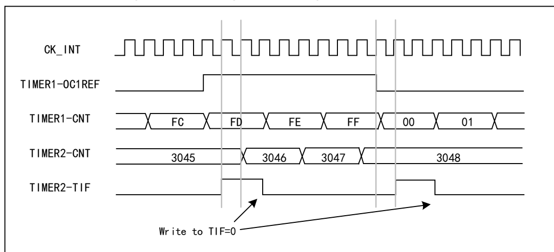
Figure 12-11 Gating Timer 2 using OC1REF of Timer 1
