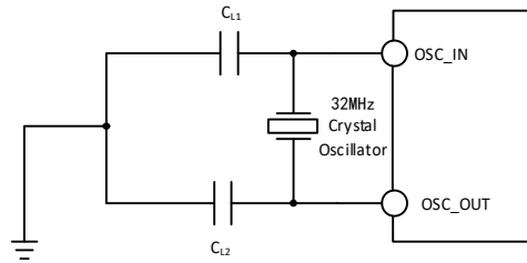
Figure 4-5 Typical circuit of external 32M crystal
