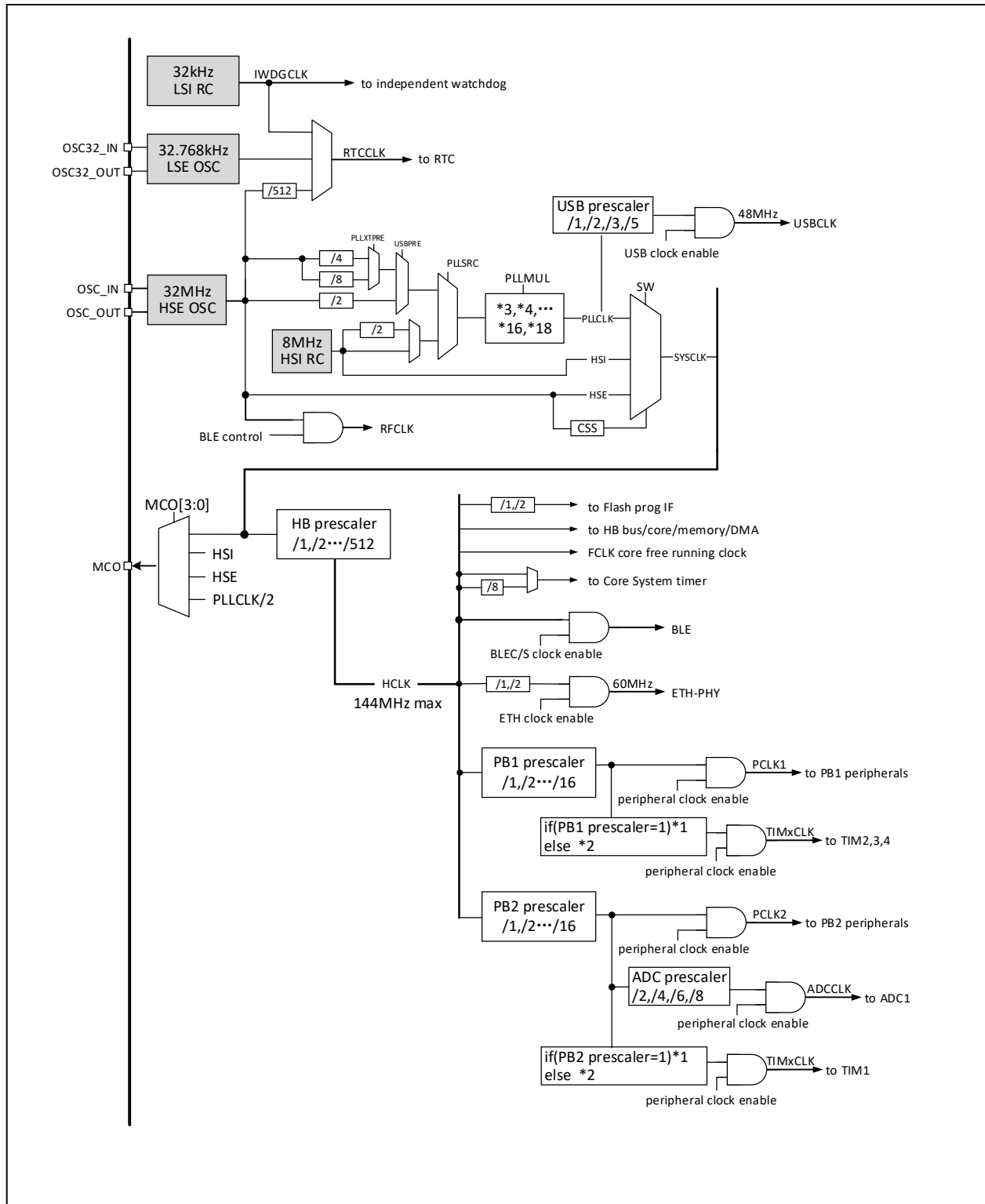
Figure 2-3 CH32V208 clock tree block diagram
