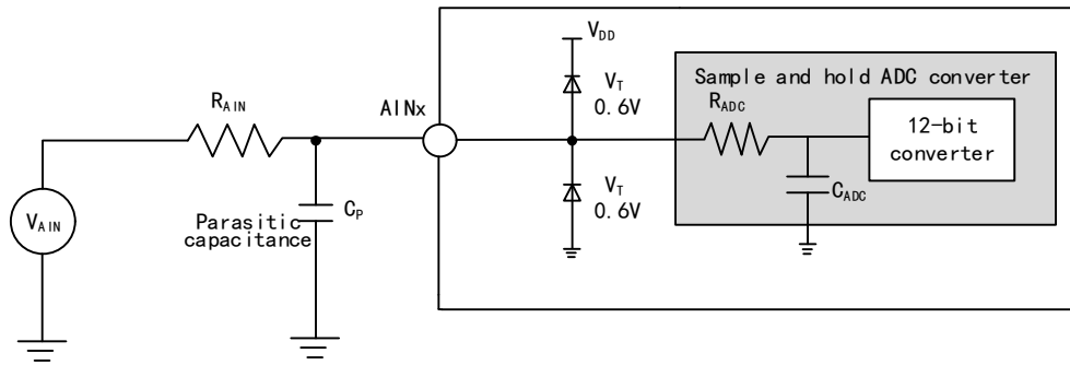
Figure 4-12 ADC typical connection diagram
