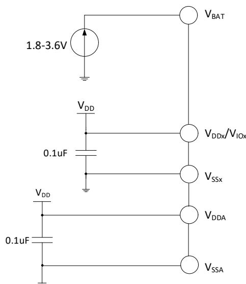
Figure 4-1 Typical circuit for conventional power supply
