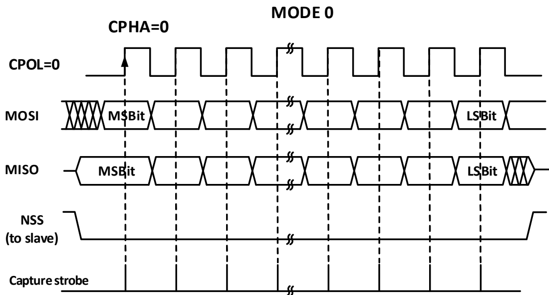
Figure 16-2 SPI master mode read/write mode 0
