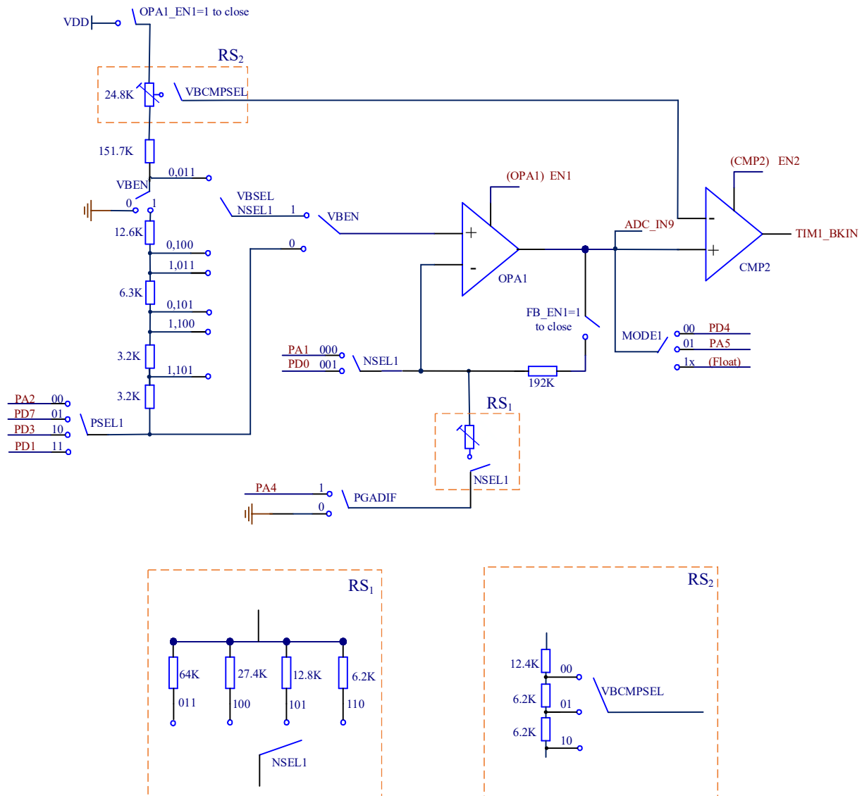
Figure 17-1 OPA structure diagram
