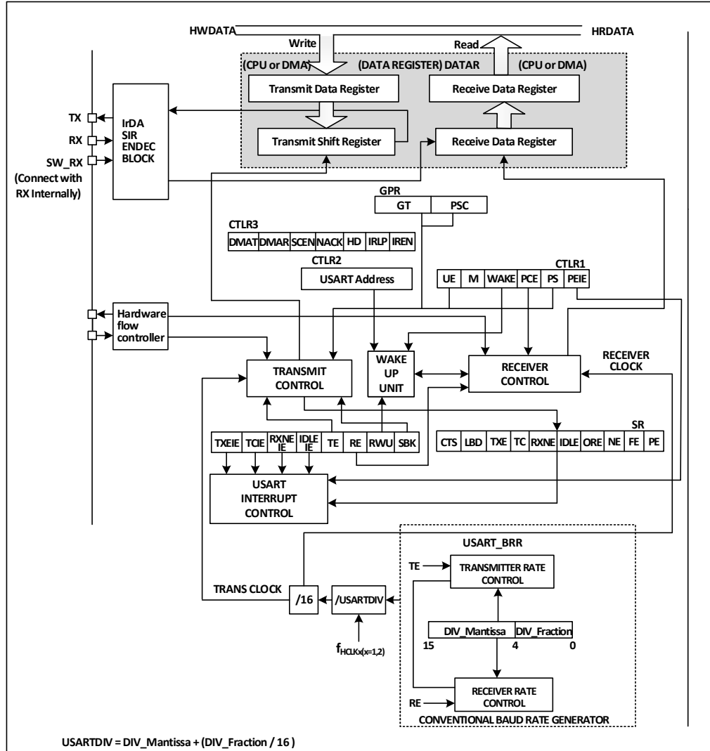
Figure 14-1 Block diagram of synchronous/asynchronous transceiver
