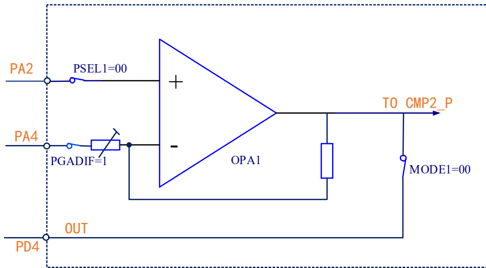
Figure 17-4 Schematic diagram of OPA differential input
