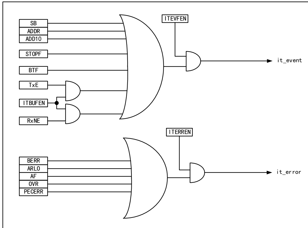
Figure 15-8 I2C Interrupt Request
