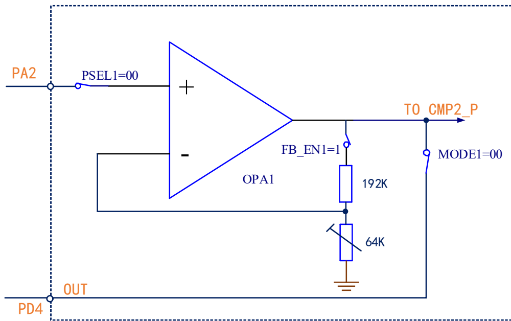
Figure 17-3 Schematic diagram of OPA internal programmable PGA
