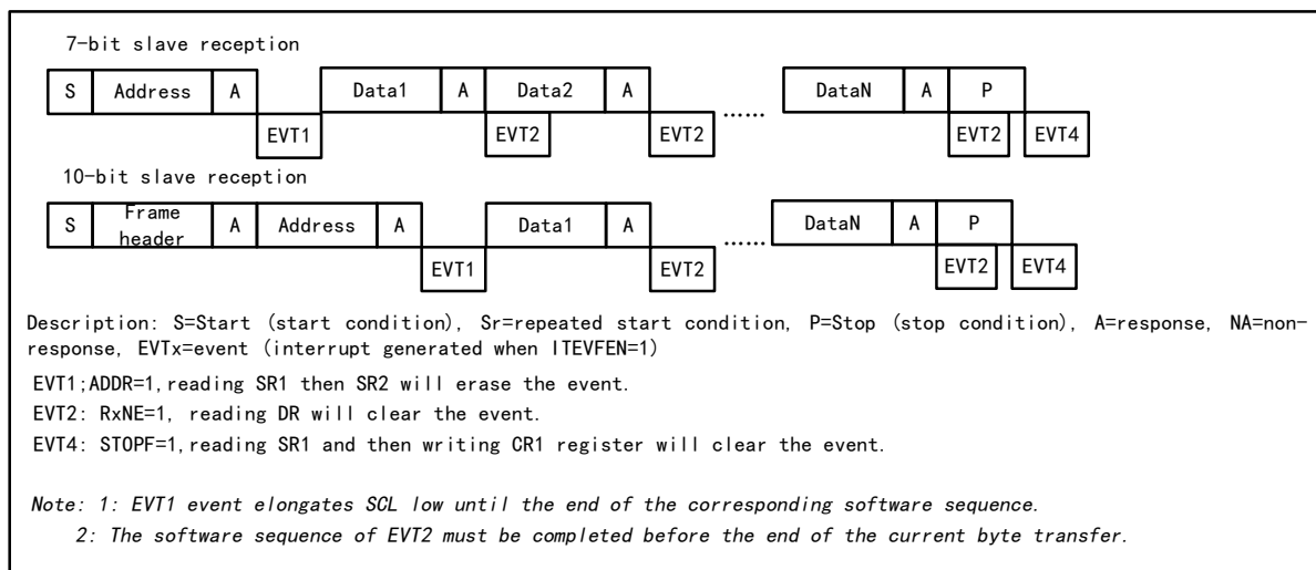
Figure 15-7 Receiver transmission sequence diagram
