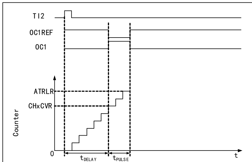
Figure 12-4 Event generation and impulse response
