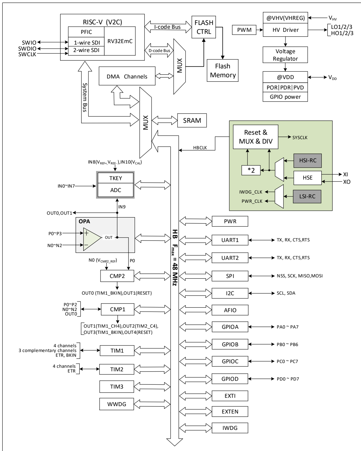
Figure 1-5-3 CH32M007E8R6 system block diagram
