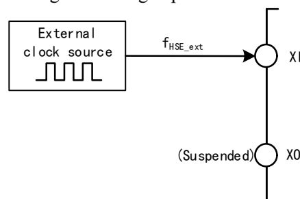
Figure 3-6 High-speed clock source circuit
