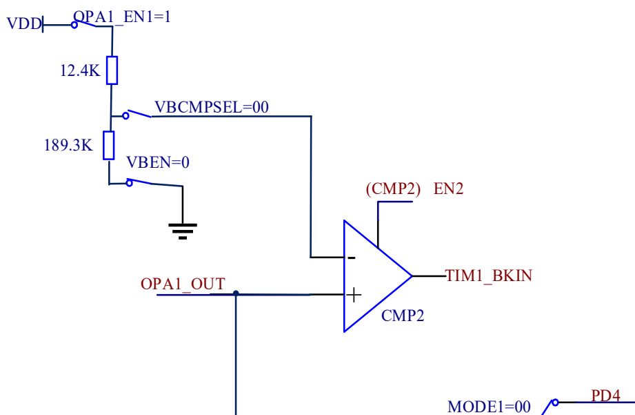
Figure 17-6 Schematic diagram of CMP2 independent bias mode
