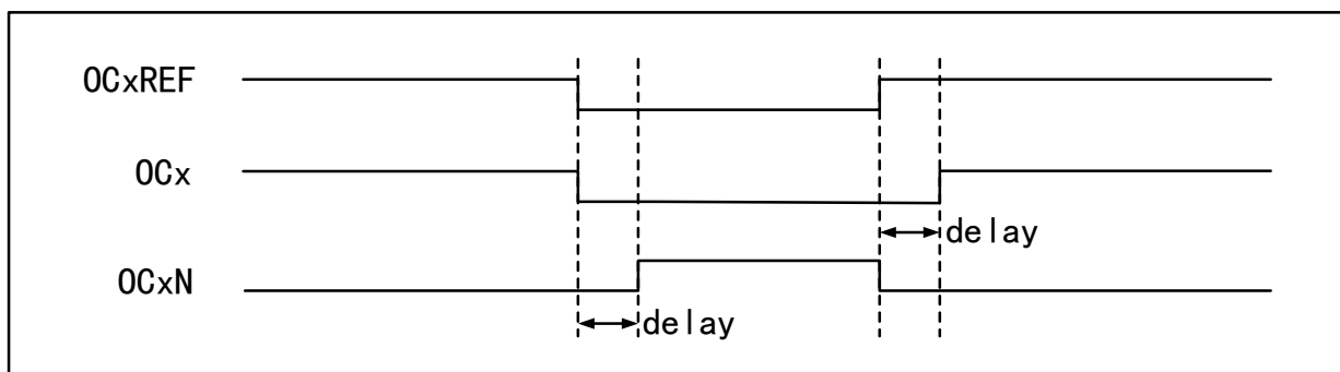
Figure 11-4 Complementary outputs and dead-time
