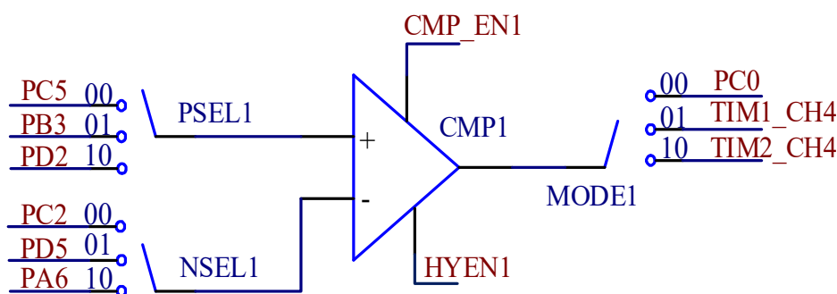
Figure 17-9 CMP structure diagram
