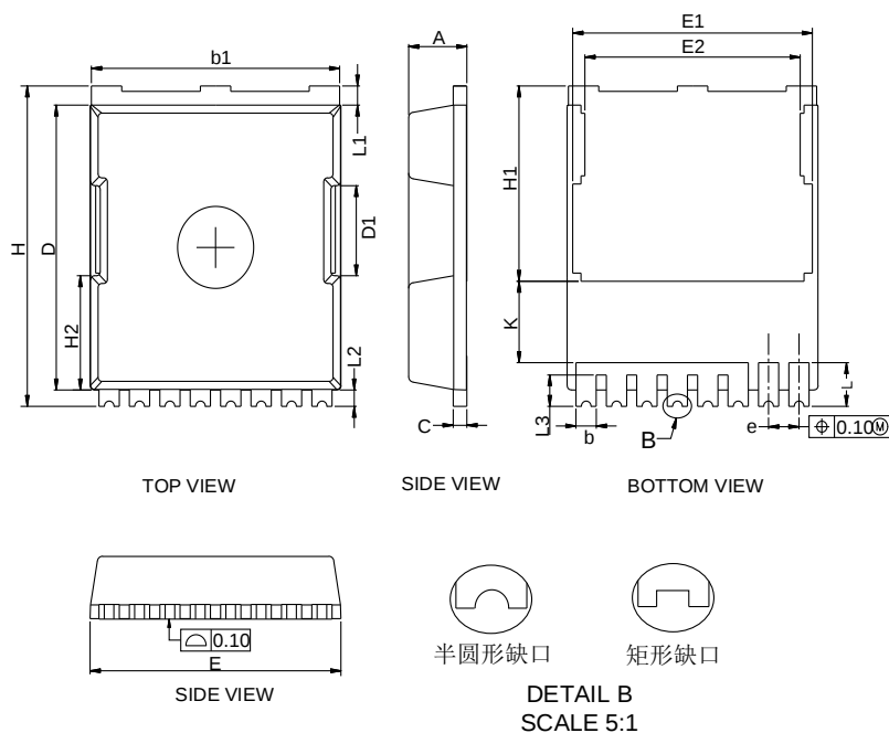
TOLL-8BL
