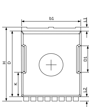
TOLL-8L
