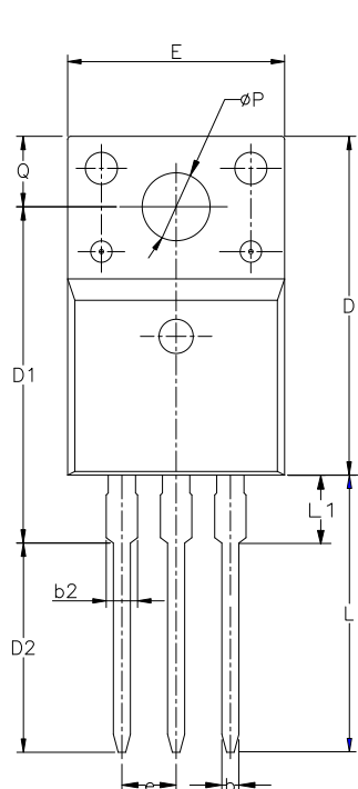
TO-220FJH-3L
