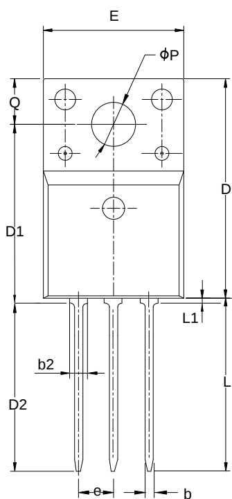
TO-220FJH-3L
