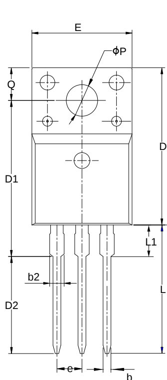
TO-220FJH-3L
