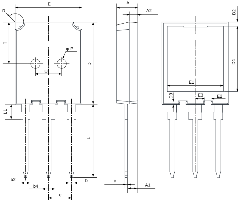
TO-247PD-3L
