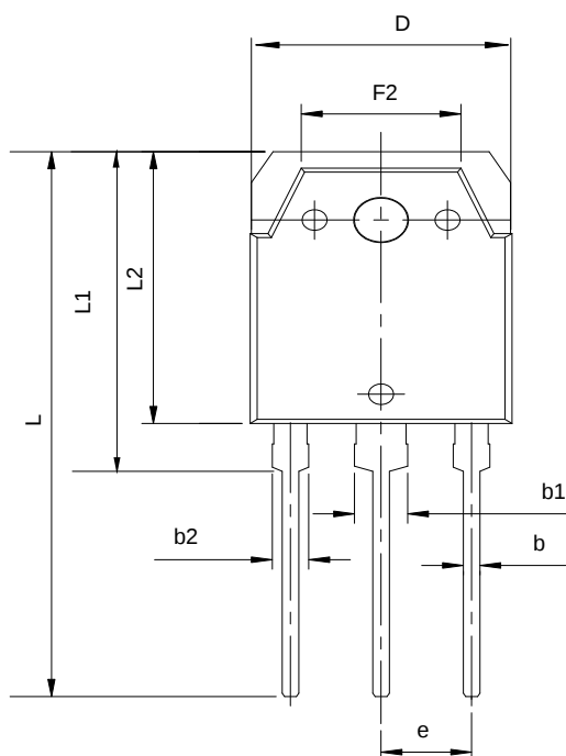
TO-3P
