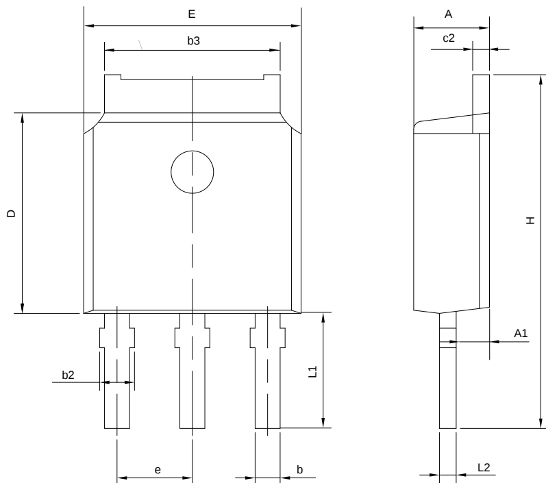
TO-220F-3L
