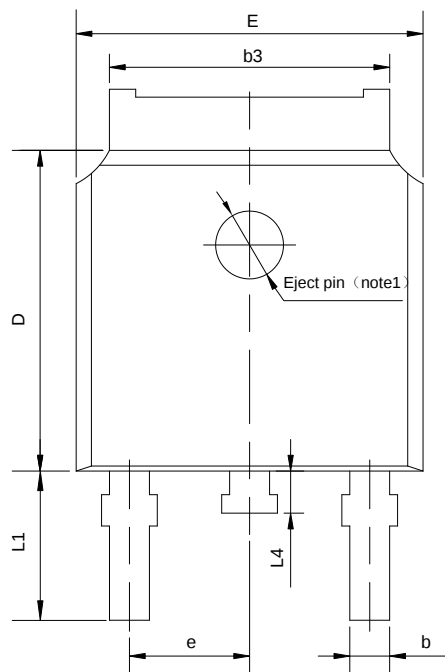
TO-252-2L
