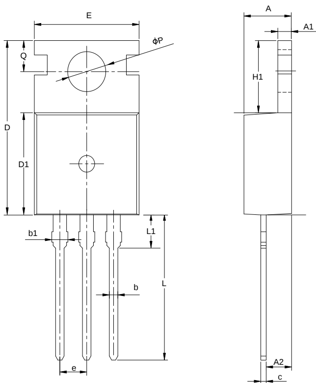
TO-220F-3L
