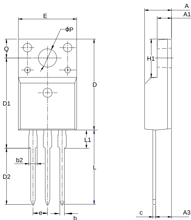
TO-220F-3L
