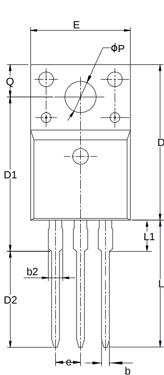
TO-220F-3L
