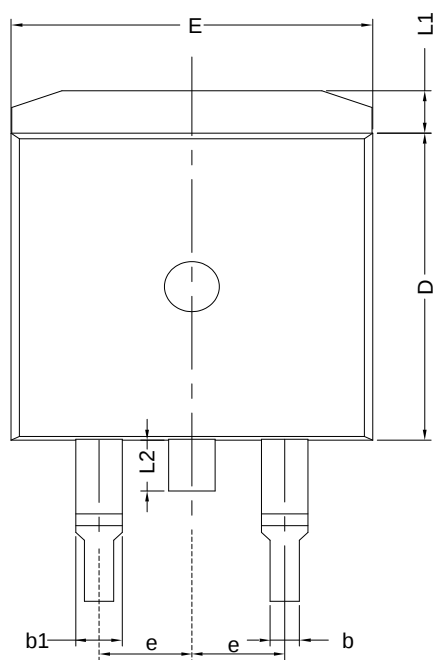
TO-262-3L
