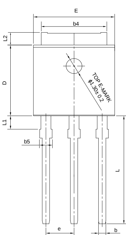
TO-251J-3L
