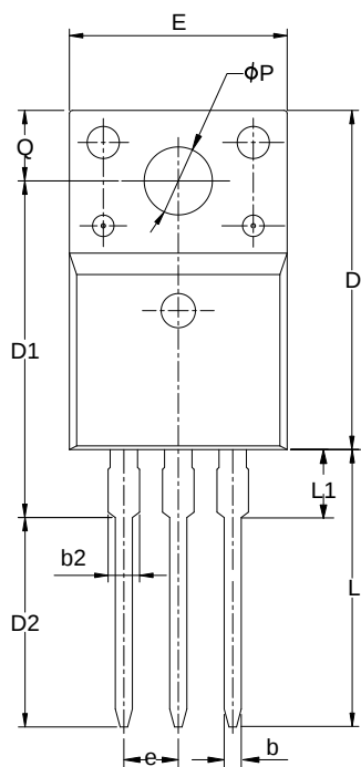
TO-220FJD-3L
