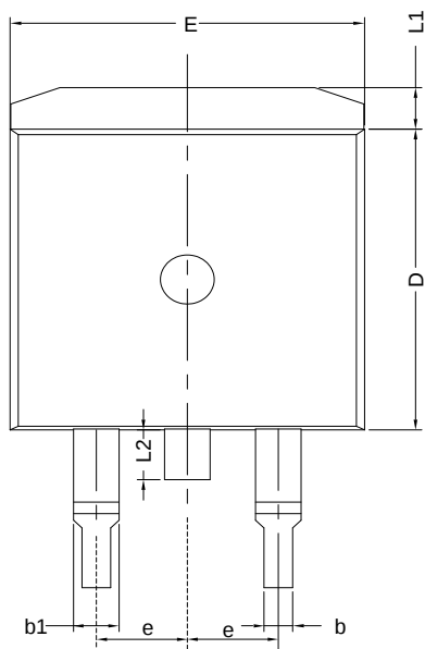
TO-220FJD-3L
