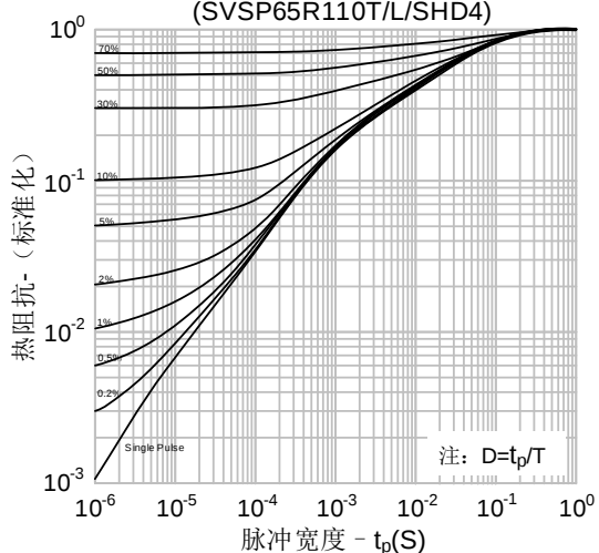
图16-2.瞬态热阻抗 vs. 脉冲宽度 (SVSP65R110T/L/SHD4)
