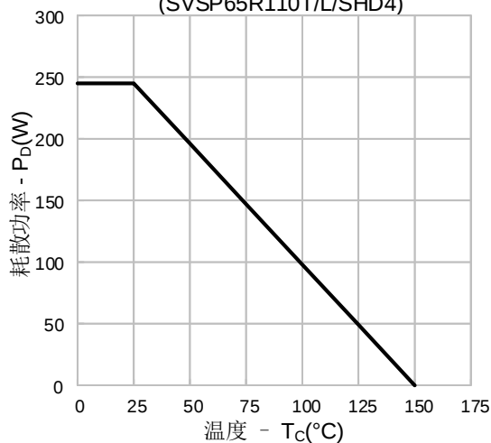
图14-2. 耗散功率vs.温度 (SVSP65R110T/L/SHD4)
