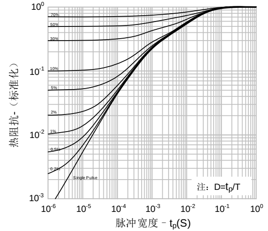
图14-1. 瞬态热阻抗 vs. 脉冲宽度(SVGP103R1NT)
