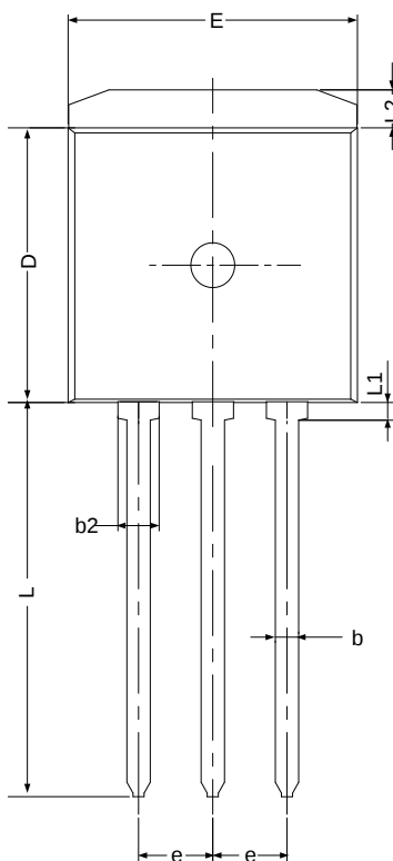
TO-262-3L
