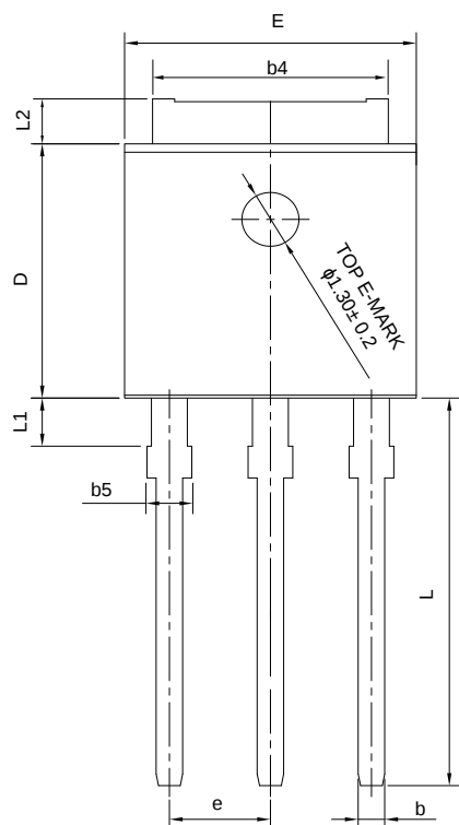
TO-251J-3L
