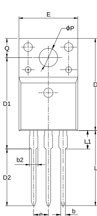
TO-220FJD-3L
