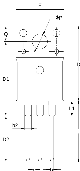
TO-220FJ-3L
