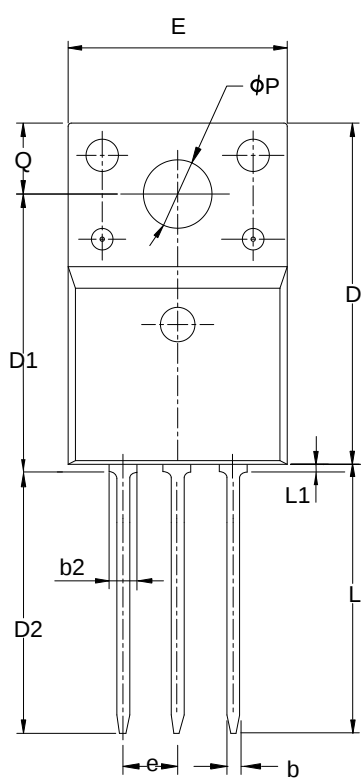
TO-220FJH-3L
