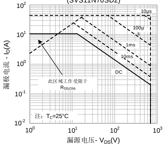
Figure 9-3. Max. Safe Operating Area (SVS11N70SD2)
