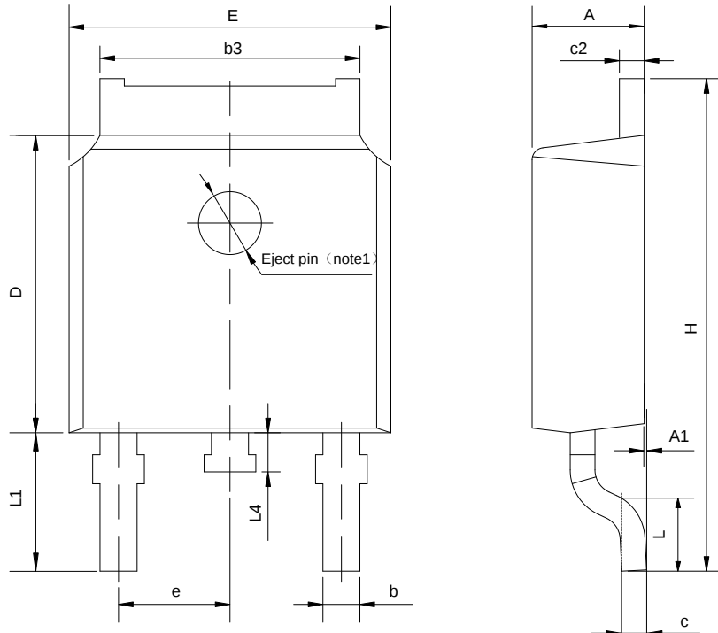
TO-252-2L
