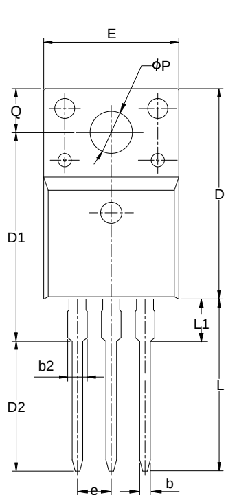
TO-220FJH-3L
