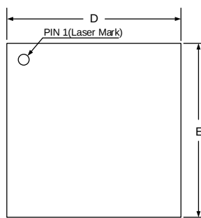
DFN-4-8x8x0.85-2.0
