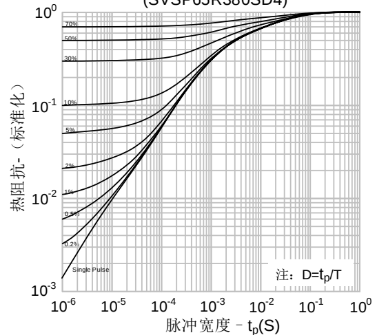
图16-3. 瞬态热阻抗 vs. 脉冲宽度 (SVSP65R380SD4)
