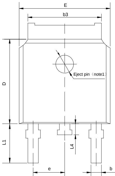
TO-252-2L
