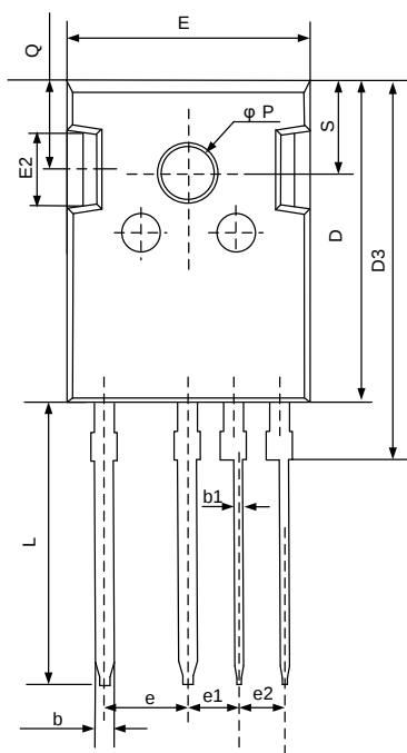
TO-247N-4L
