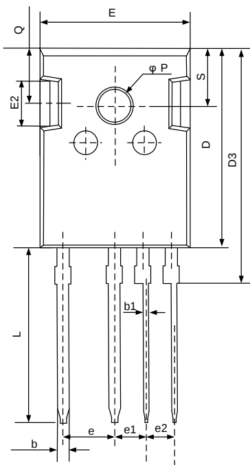
TO-247N-4L
