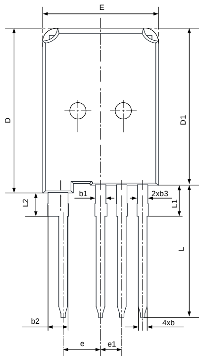
TO-247PJ-4L
