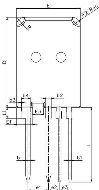
TO-247PJ-4L
