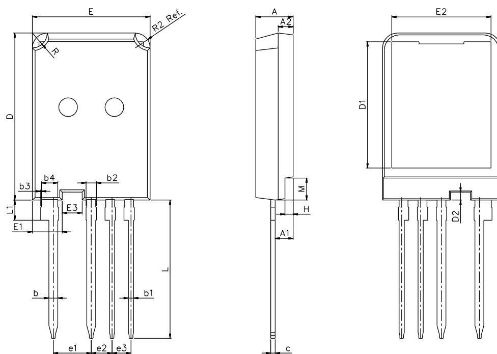
TO-247PJ-4L
