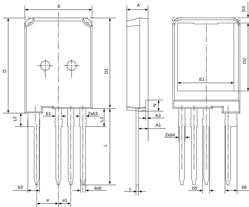
TO-247PJ-4L
