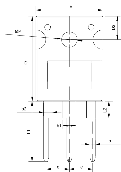
TO-247S-3L
