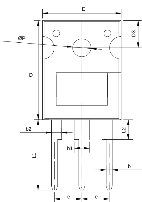
TO-3PN
