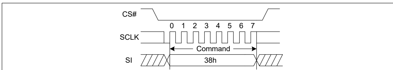
Figure 69. Enable QPI mode command Sequence Diagram
