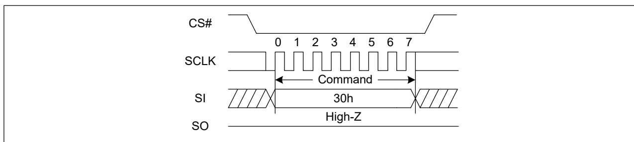
Figure 17. Clear Status Register Flags Sequence Diagram
