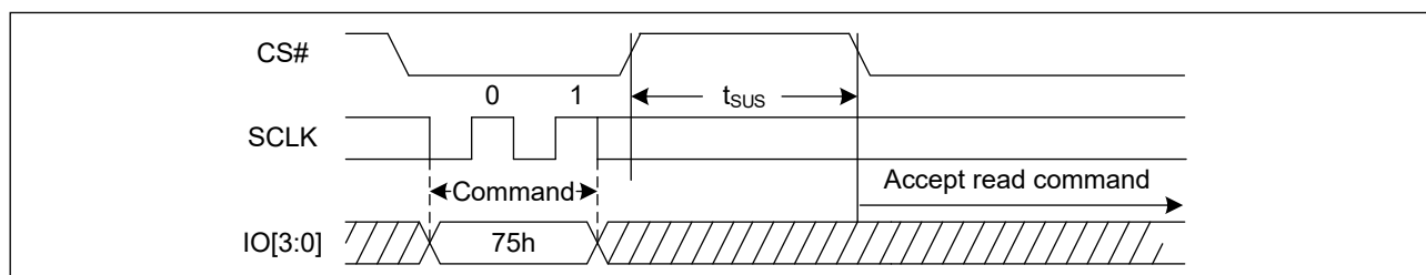
Figure 60. Program/Erase Suspend Sequence Diagram (QPI)
