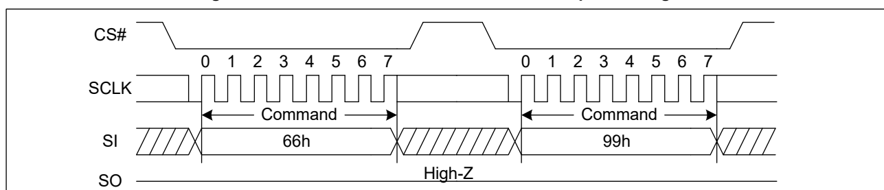
Figure 33. Enable Reset and Reset command Sequence Diagram
