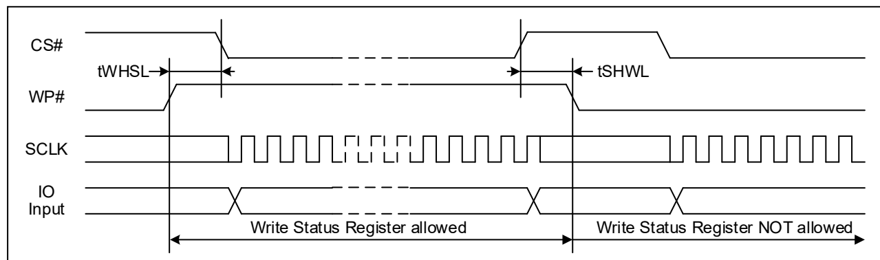
Figure 48. WP# Timing
