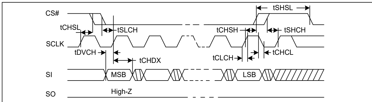
Figure 64. Input Timing
