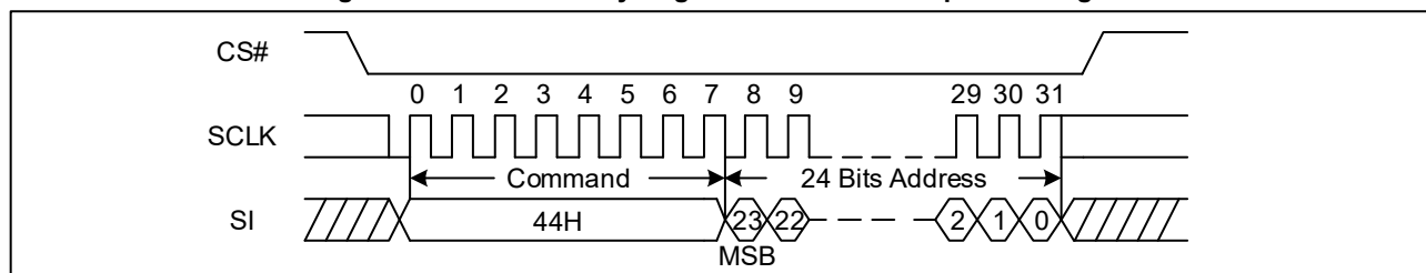
Figure 41. Erase Security Registers command Sequence Diagram
