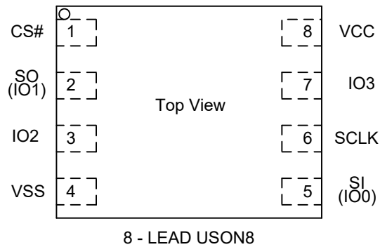
Figure 1. Connection Diagram for USON8 package
