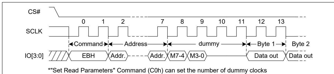
Figure 22 Quad I/O Fast Read Sequence Diagram (M5-4 = (1, 0))
