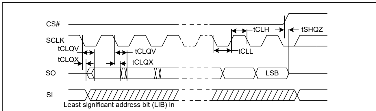
Figure 65. Output Timing
