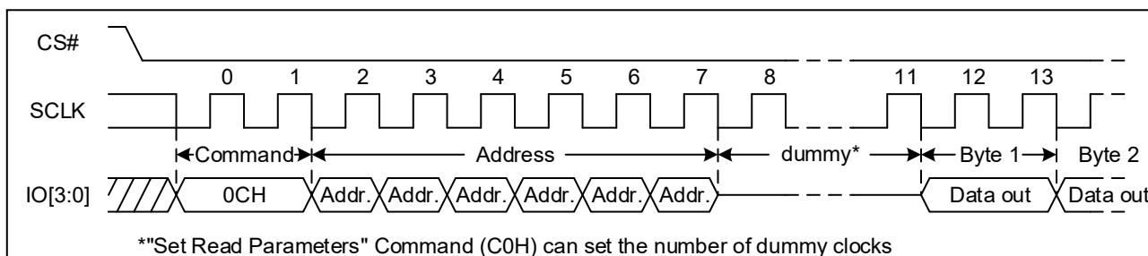
Figure 46. Burst Read with Wrap command Sequence Diagram
