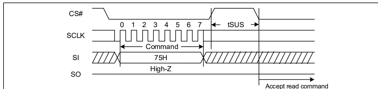
Figure 47. Program/Erase Suspend Sequence Diagram (SPI)
