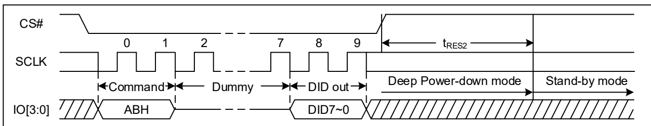
Figure 56. Release Power-Down/Read Device ID Sequence Diagram (QPI)
