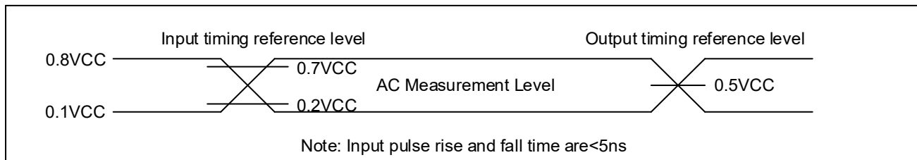
Figure 63. Absolute Maximum Ratings Diagram
