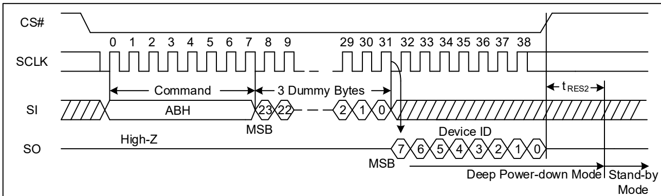
Figure 55. Release Power-Down/Read Device ID Sequence Diagram (SPI)
