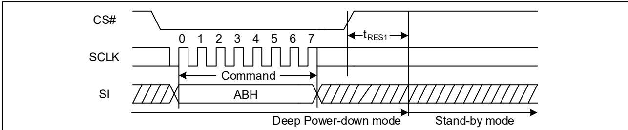
Figure 53. Release Power-Down Sequence Diagram (SPI)
