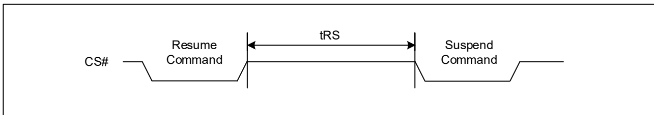
Figure 66. Resume to Suspend Timing Diagram
