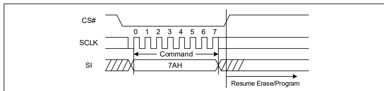
Figure 49. Program/Erase Resume Sequence Diagram (SPI)
