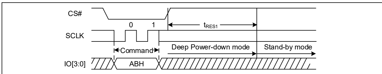
Figure 54. Release Power-Down Sequence Diagram (QPI)
