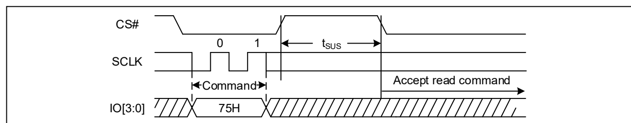
Figure 48. Program/Erase Suspend Sequence Diagram (QPI)
