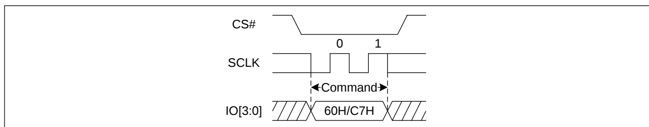
Figure 36. Chip Erase Sequence Diagram (QPI)
