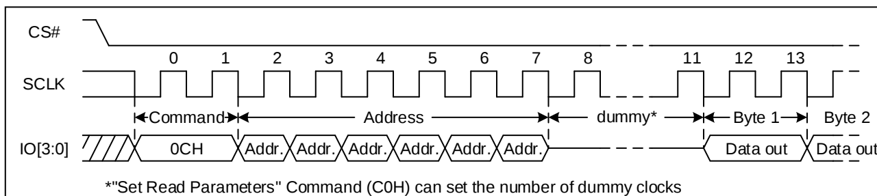
Figure 48. Burst Read with Wrap command Sequence Diagram
