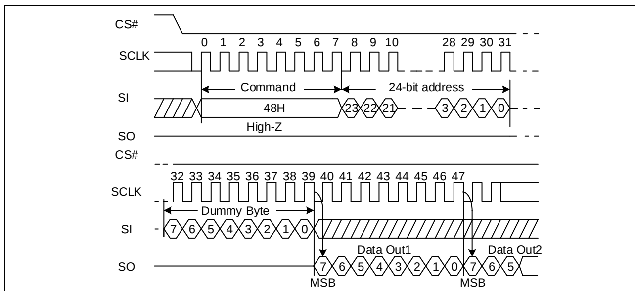
Figure 45. Read Security Registers command Sequence Diagram
