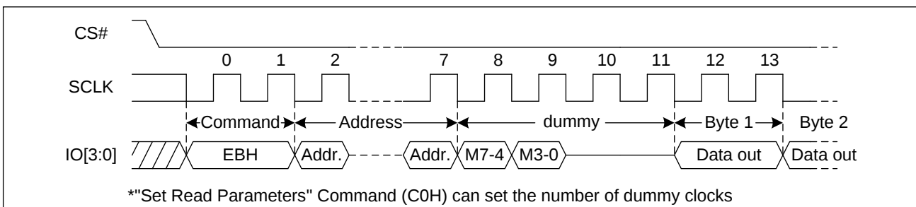
Figure 21 Quad I/O Fast Read Sequence Diagram (M5-4 = (1, 0))
