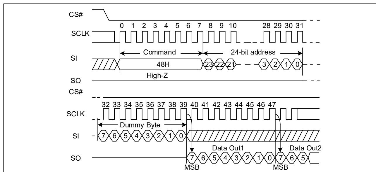
Figure 48. Read Security Registers command Sequence Diagram
