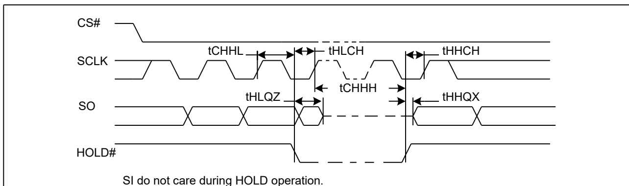
Figure 74. Hold Timing
