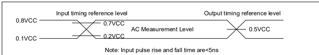
Figure 68. Absolute Maximum Ratings Diagram
