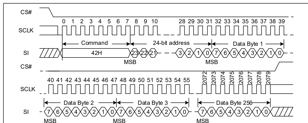
Figure 47. Program Security Registers command Sequence Diagram
