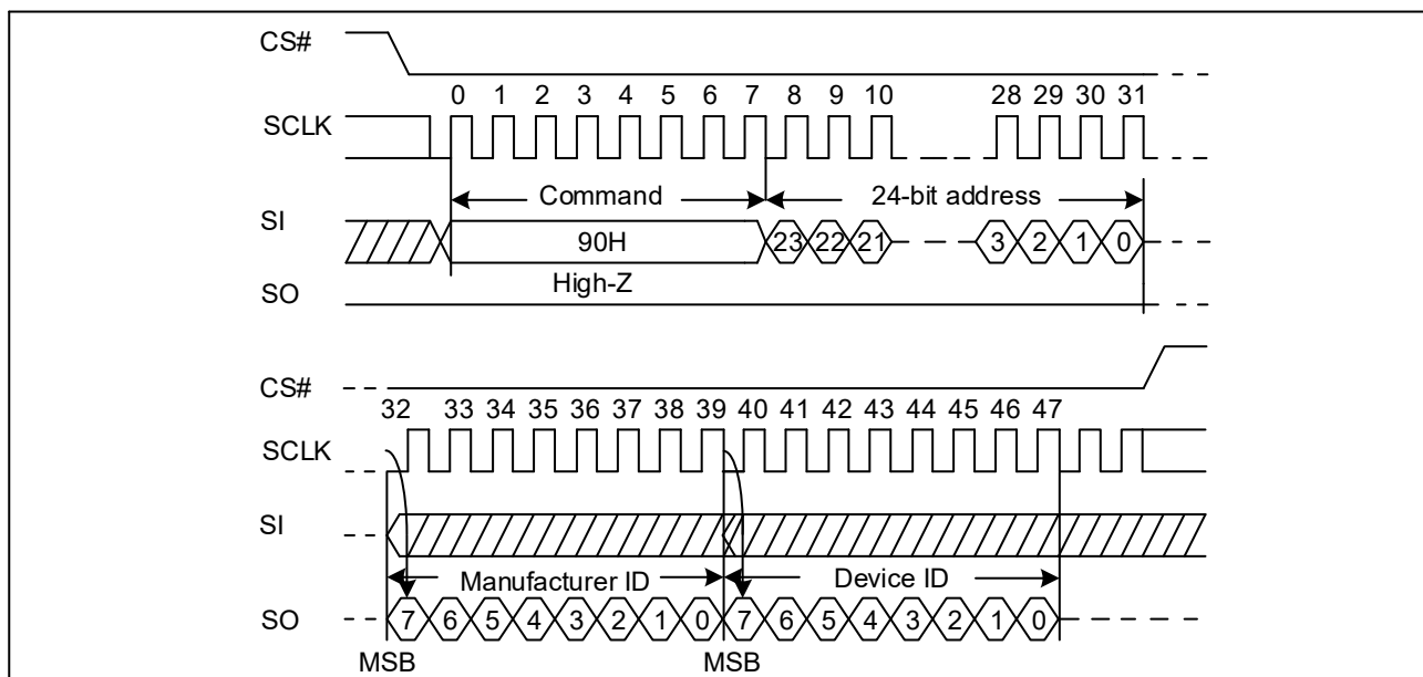
Figure 41. Read Manufacture ID/ Device ID Sequence Diagram (SPI)
