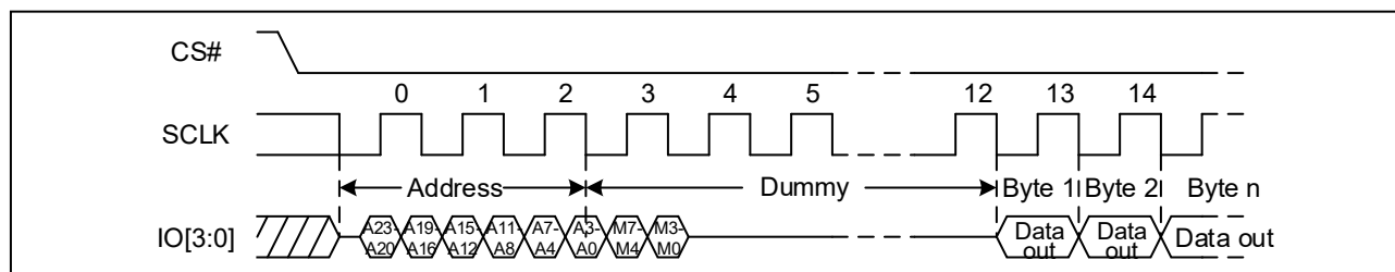
Figure 27. DTR Quad I/O Fast Read Sequence Diagram ((M5-4) = (1, 0))
