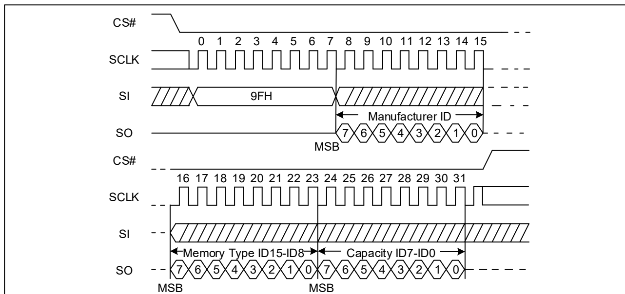
Figure 43. Read Identification ID Sequence Diagram (SPI)
