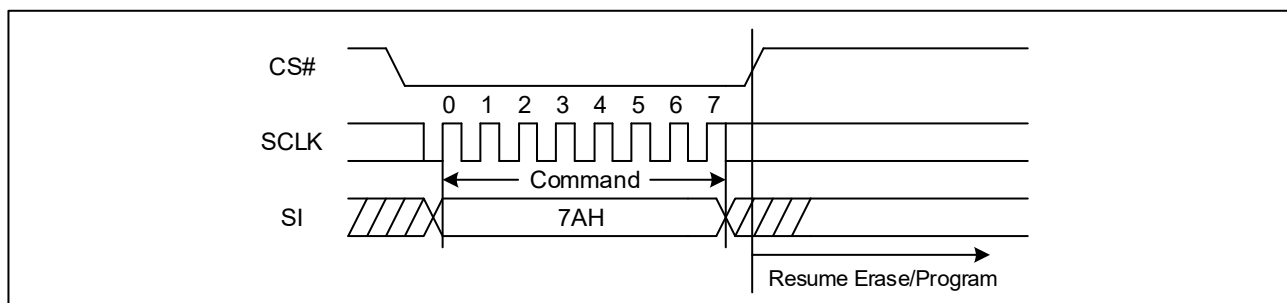
Figure 54. Program/Erase Resume Sequence Diagram (SPI)
