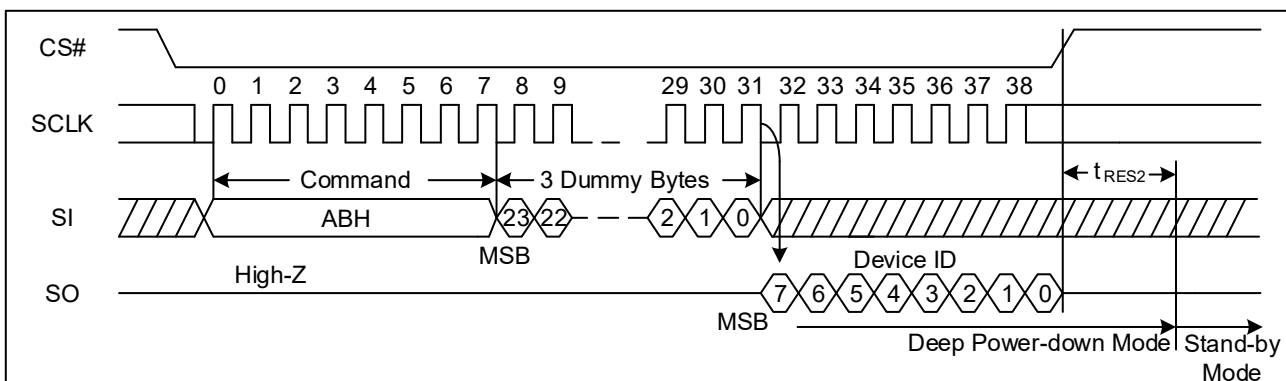
Figure 60. Release Power-Down/Read Device ID Sequence Diagram (SPI)
