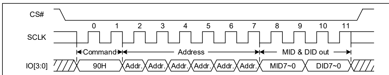
Figure 42. Read Manufacture ID/ Device ID Sequence Diagram (QPI)
