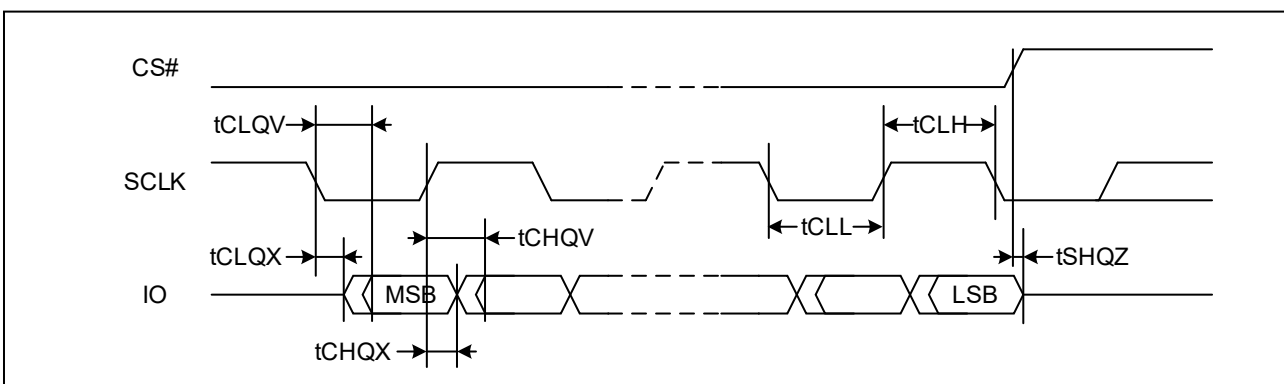
Figure 72. Serial Output Timing (DTR)
