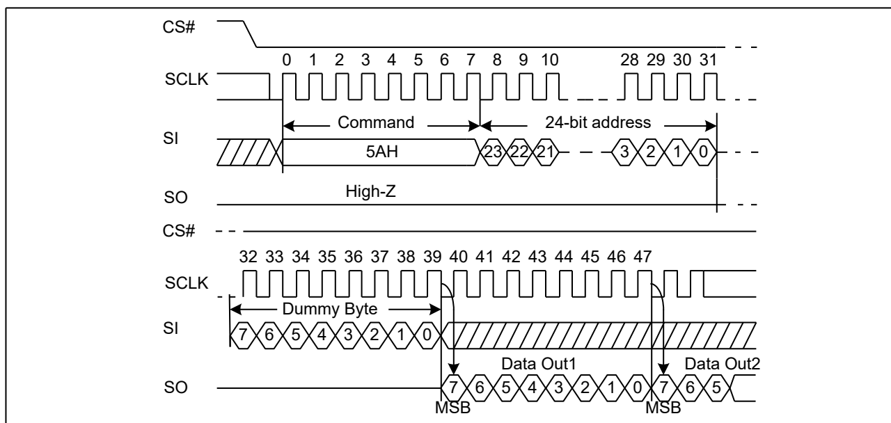
Figure 64. Read Serial Flash Discoverable Parameter command Sequence Diagram
