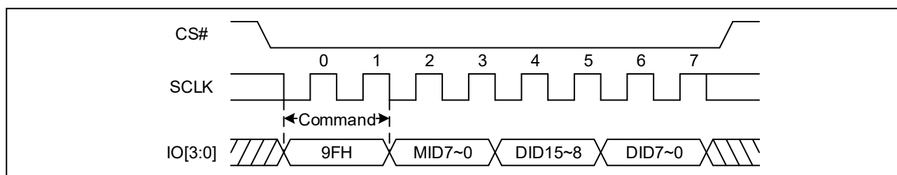
Figure 44. Read Identification ID Sequence Diagram (QPI)
