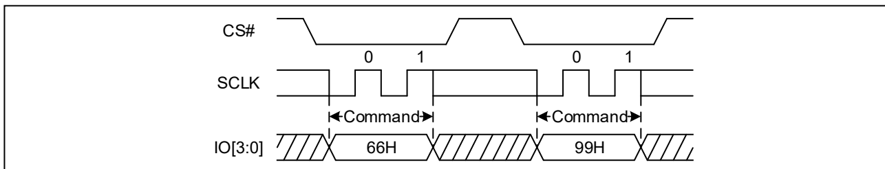
Figure 50. Enable Reset and Reset command Sequence Diagram (QPI)
