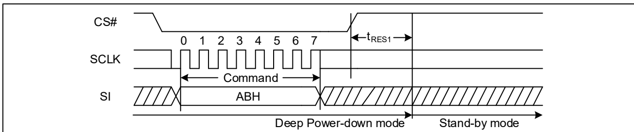
Figure 58. Release Power-Down Sequence Diagram (SPI)
