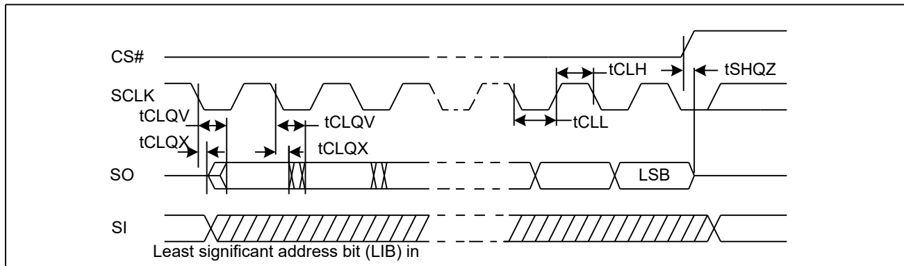
Figure 70. Output Timing
