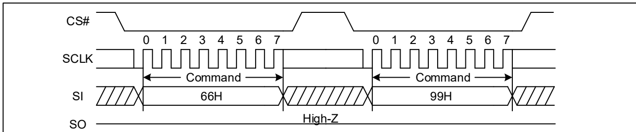
Figure 49. Enable Reset and Reset command Sequence Diagram (SPI)
