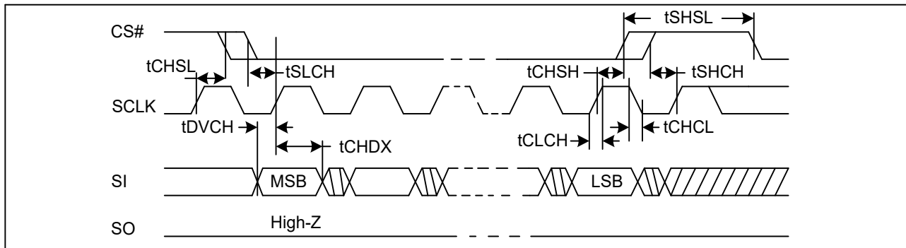
Figure 69. Input Timing
