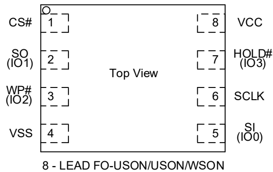
Figure 2 Connection Diagram for FO-USON8/USON8/WSON8 package
