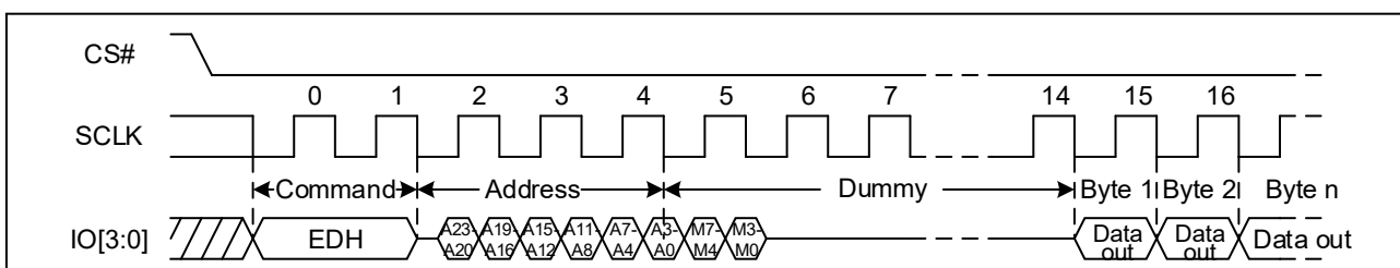
Figure 26. DTR Quad I/O Fast Read Sequence Diagram (QPI, (M5-4) ≠ (1, 0))
