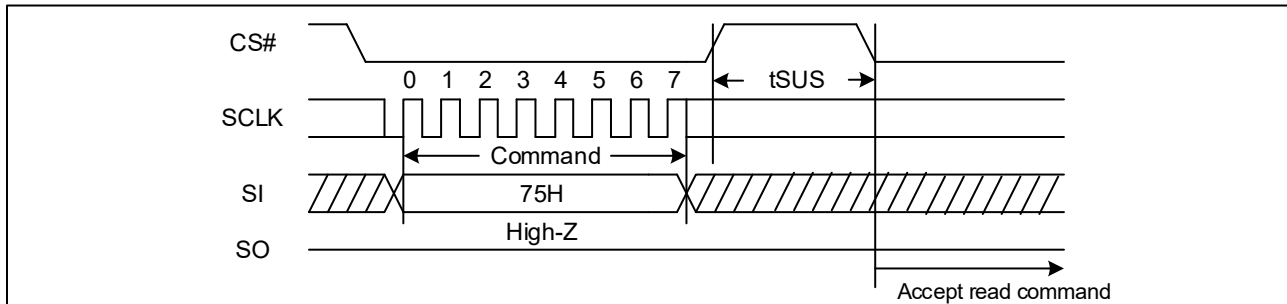
Figure 52. Program/Erase Suspend Sequence Diagram (SPI)
