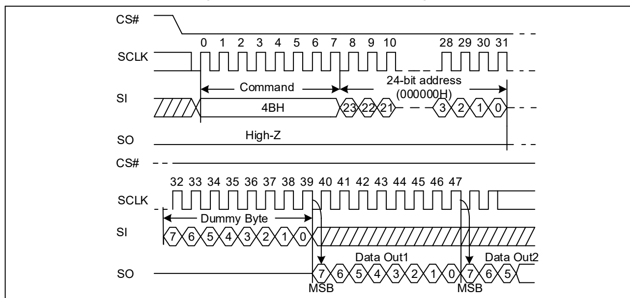
Figure 45. Read Unique ID Sequence Diagram
