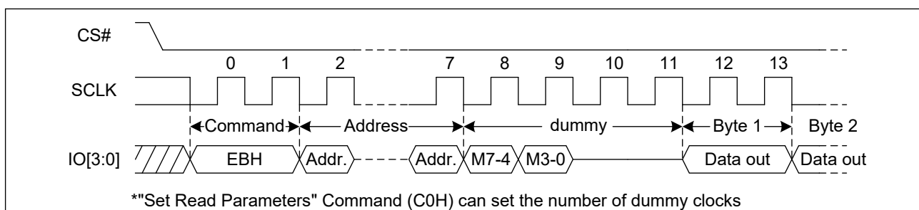
Figure 23. Quad I/O Fast Read Sequence Diagram (QPI, M5-4 ≠ (1, 0))
