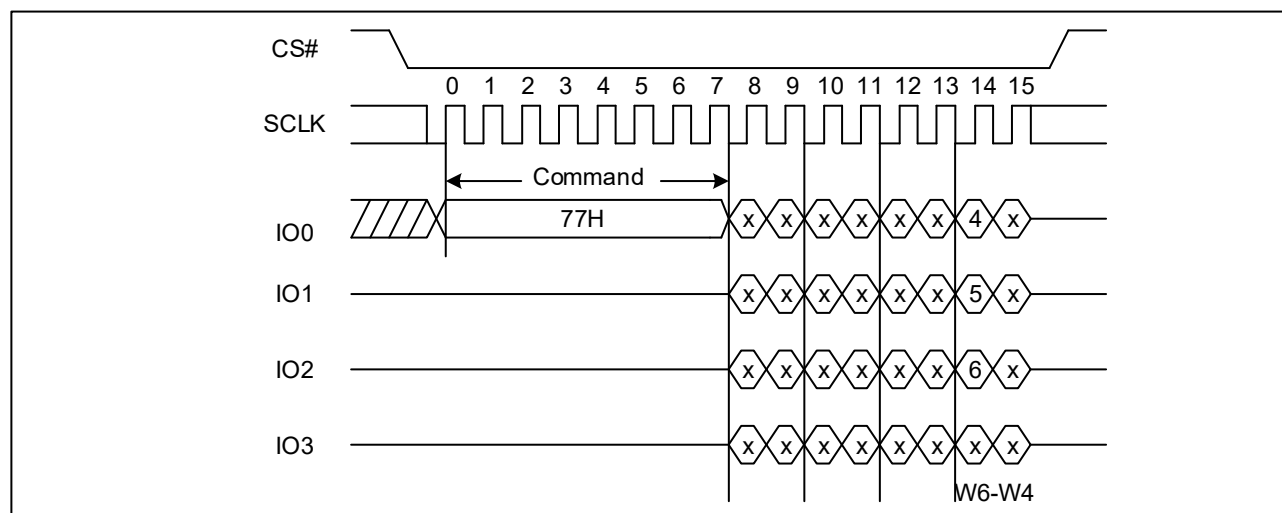
Figure 28. Set Burst with Wrap Sequence Diagram
