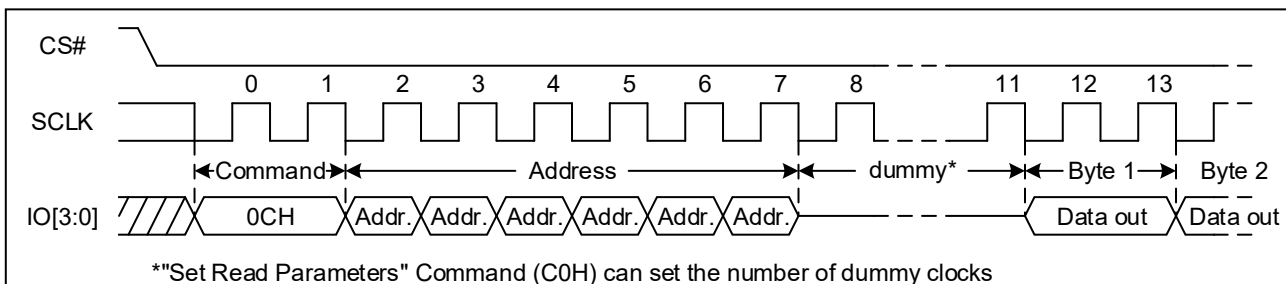
Figure 51. Burst Read with Wrap command Sequence Diagram
