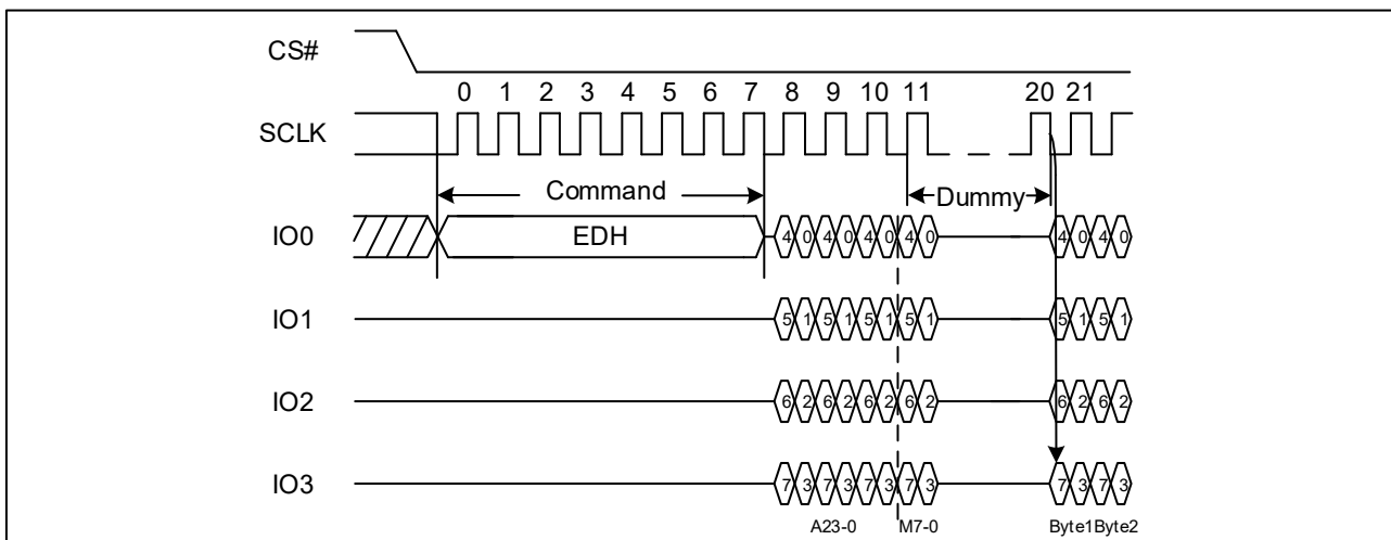
Figure 25. DTR Quad I/O Fast Read Sequence Diagram (SPI, (M5-4) ≠ (1, 0))
