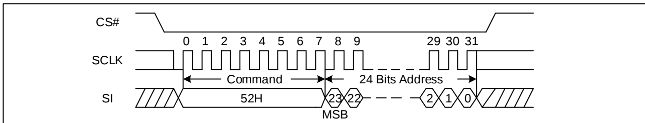
Figure 31. 32KB Block Erase Sequence Diagram (SPI)
