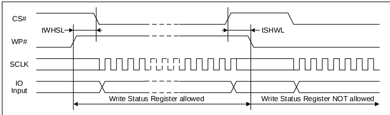
Figure 72. WP# Timing
