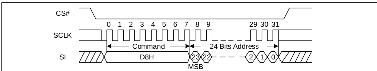
Figure 33. 64KB Block Erase Sequence Diagram (SPI)
