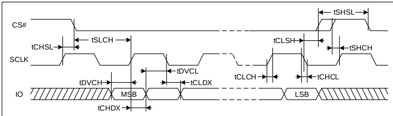
Figure 68. Serial Input Timing (DTR)
