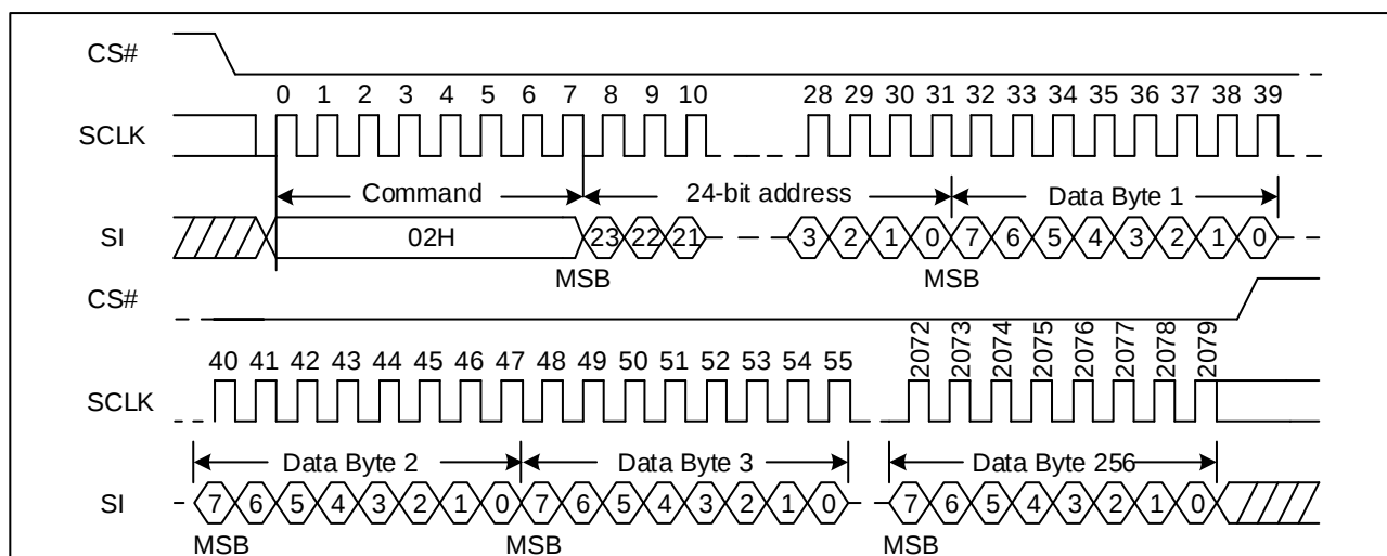
Figure 26. Page Program Sequence Diagram (SPI)
