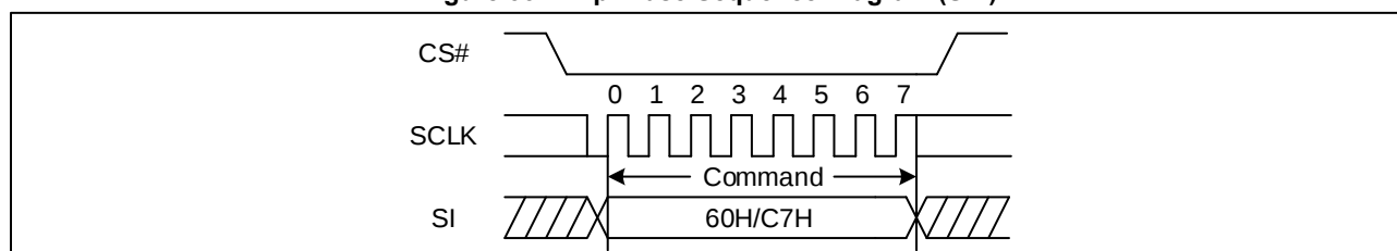
Figure 35. Chip Erase Sequence Diagram (SPI)
