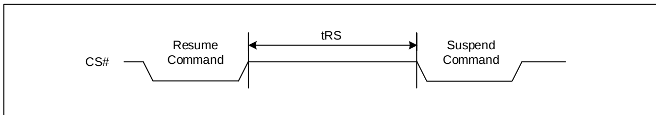
Figure 70. Resume to Suspend Timing Diagram
