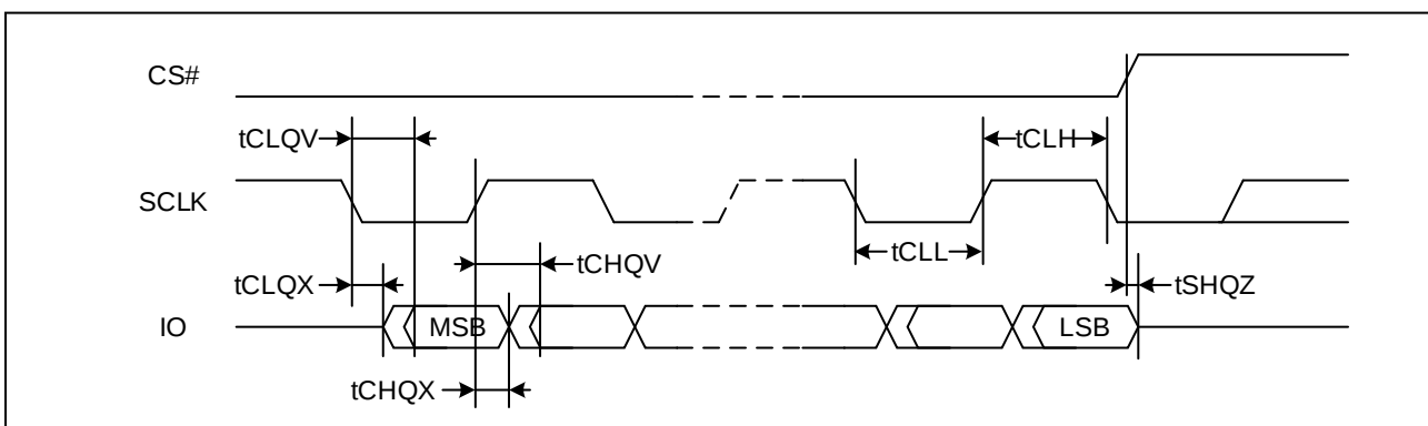
Figure 69. Serial Output Timing (DTR)
