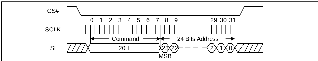
Figure 29. Sector Erase Sequence Diagram (SPI)
