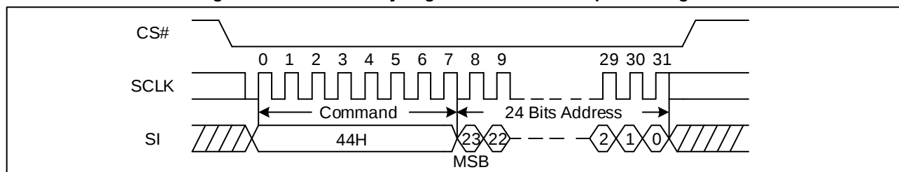
Figure 43. Erase Security Registers command Sequence Diagram
