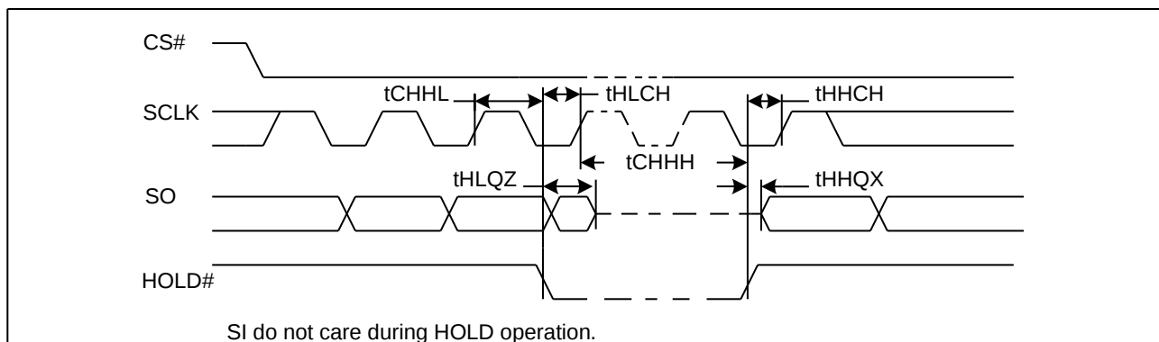
Figure 71. Hold Timing
