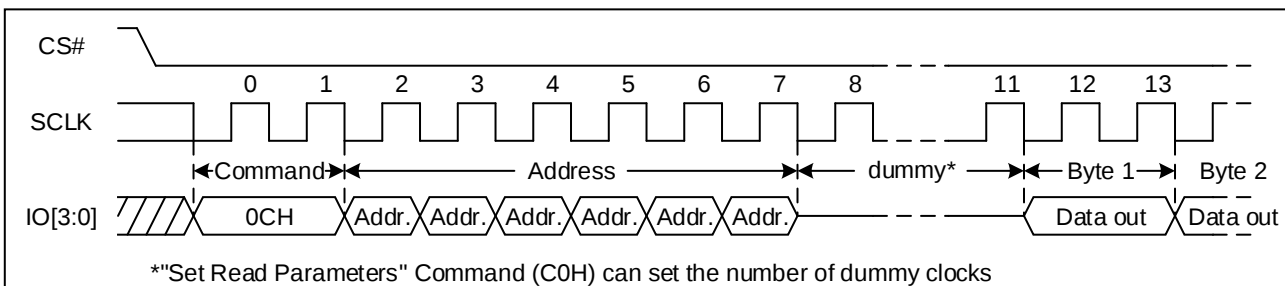
Figure 48. Burst Read with Wrap command Sequence Diagram
