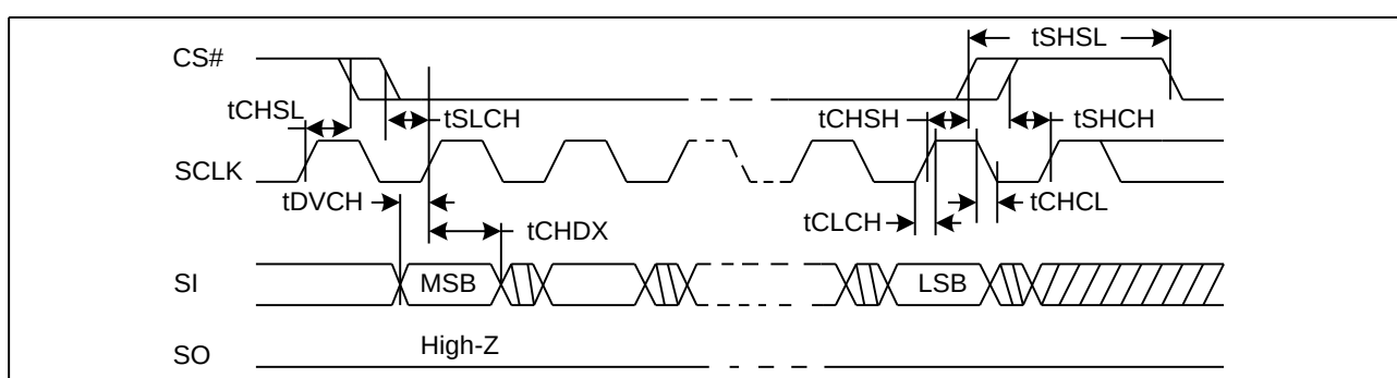
Figure 45. Output Timing
