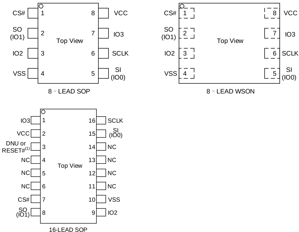
Figure 1. Connection Diagram
